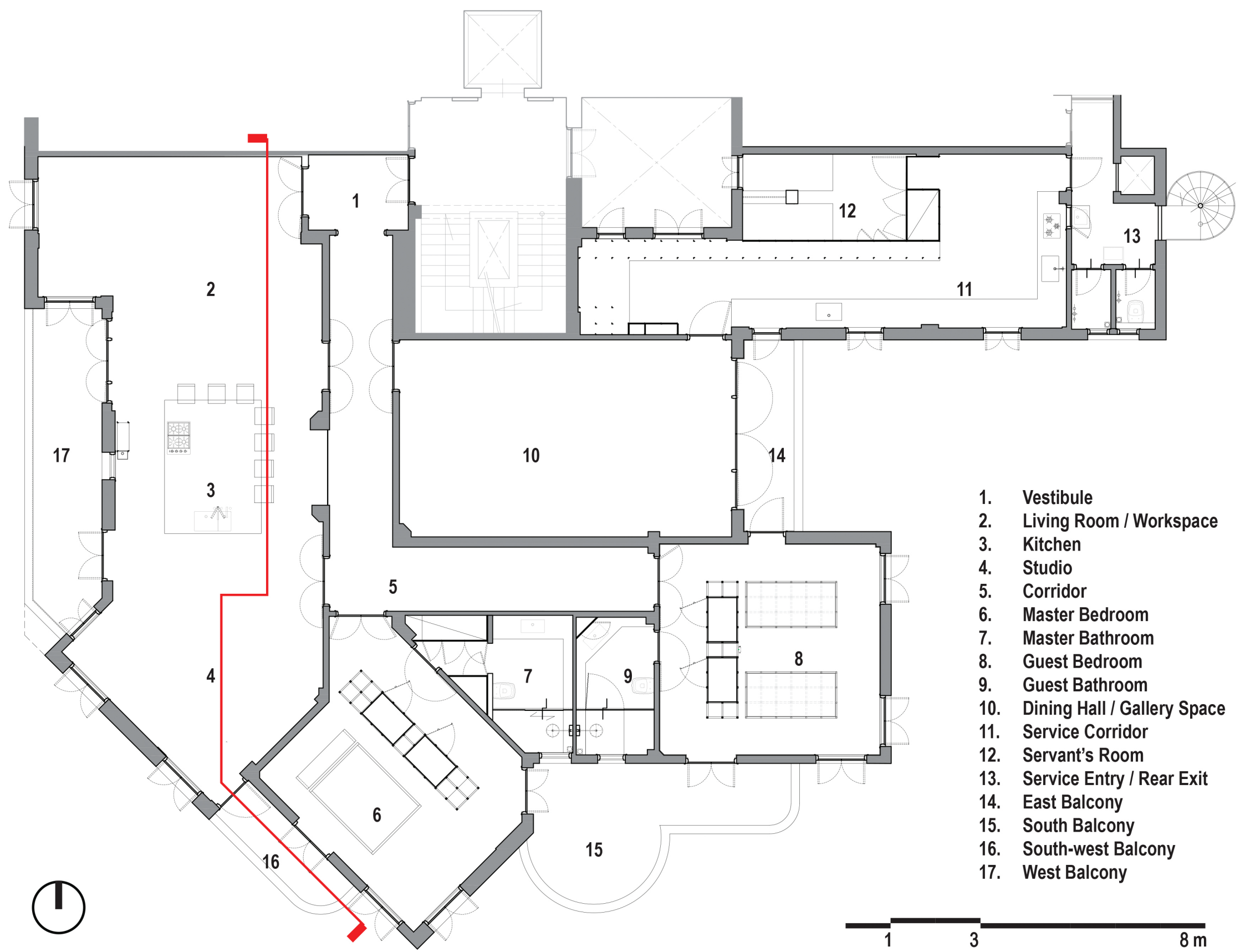
Proposed Plan
