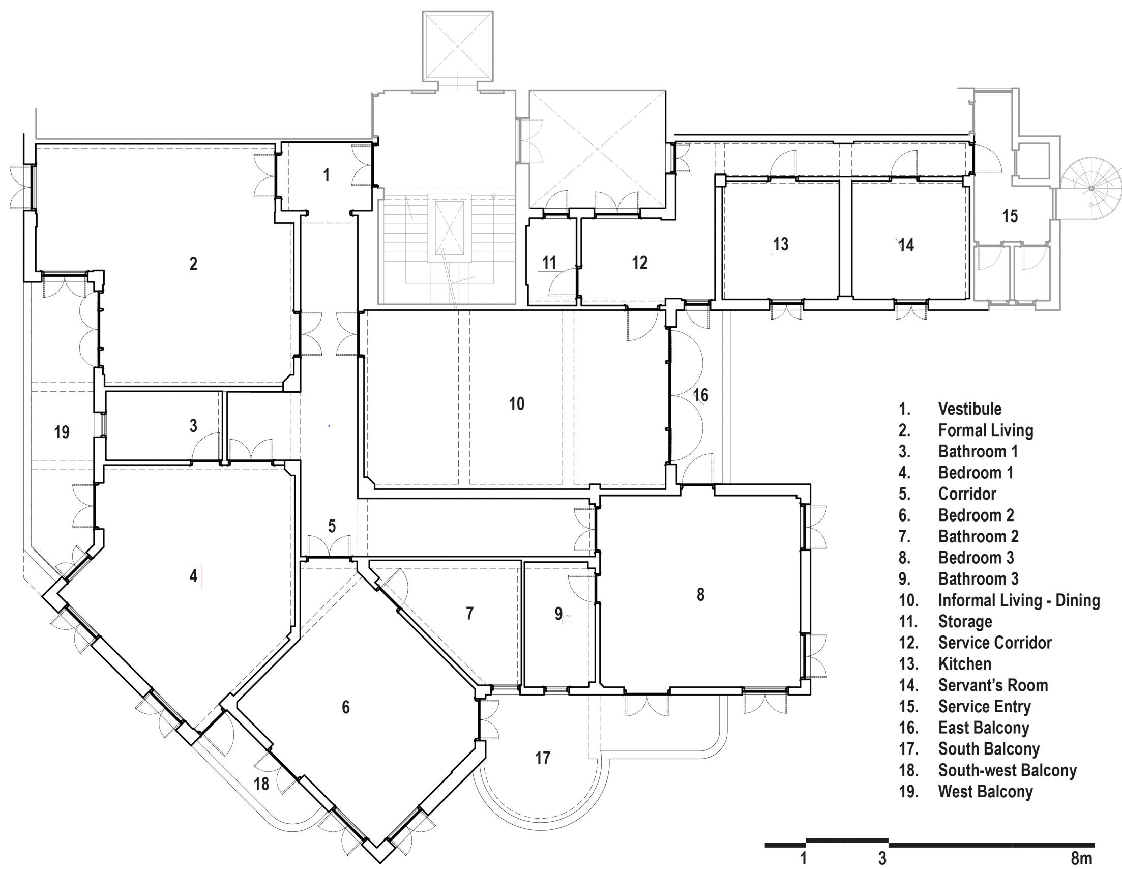
Existing Plan
