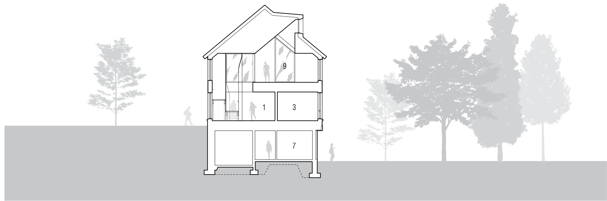
TRANSVERSE SECTION
