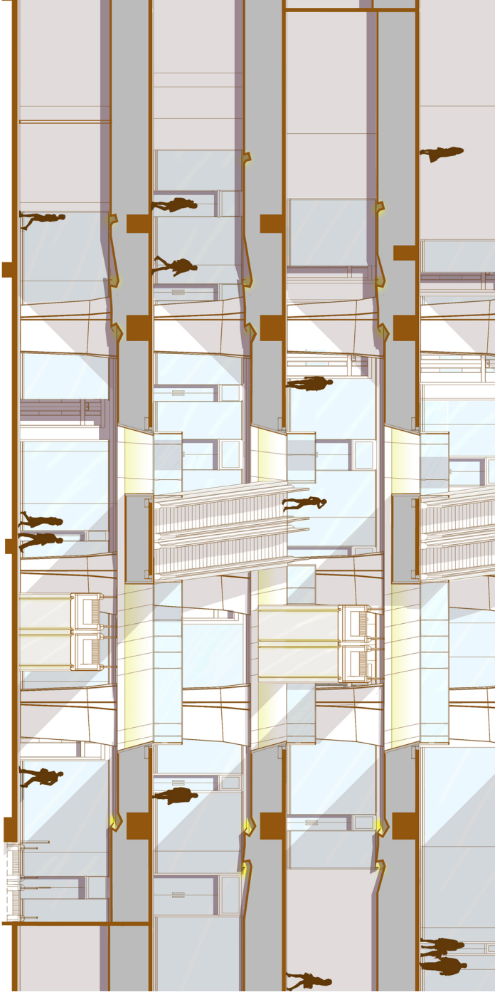
ESCALATOR LOBBY SECTION 2-2
