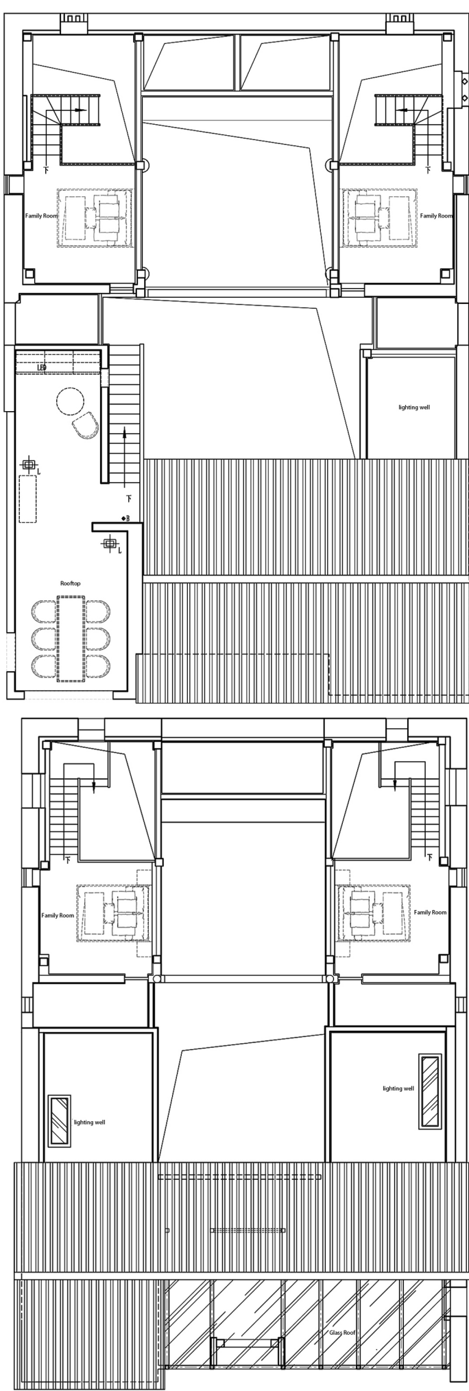
2ndFloorPlanForBuilding 1&2
