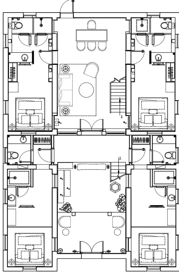
2ndFloorPlanForBuilding 3
