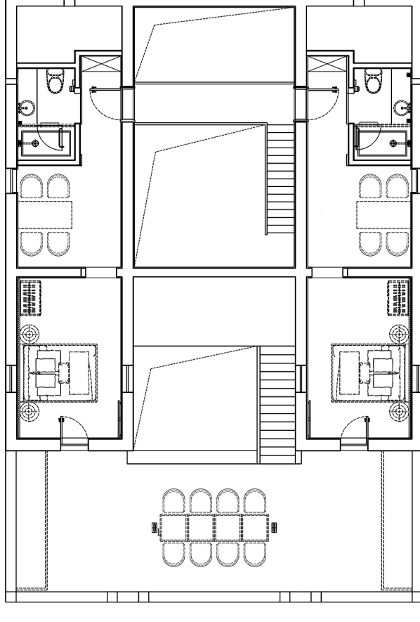
1stFloorPlanForBuilding 3
