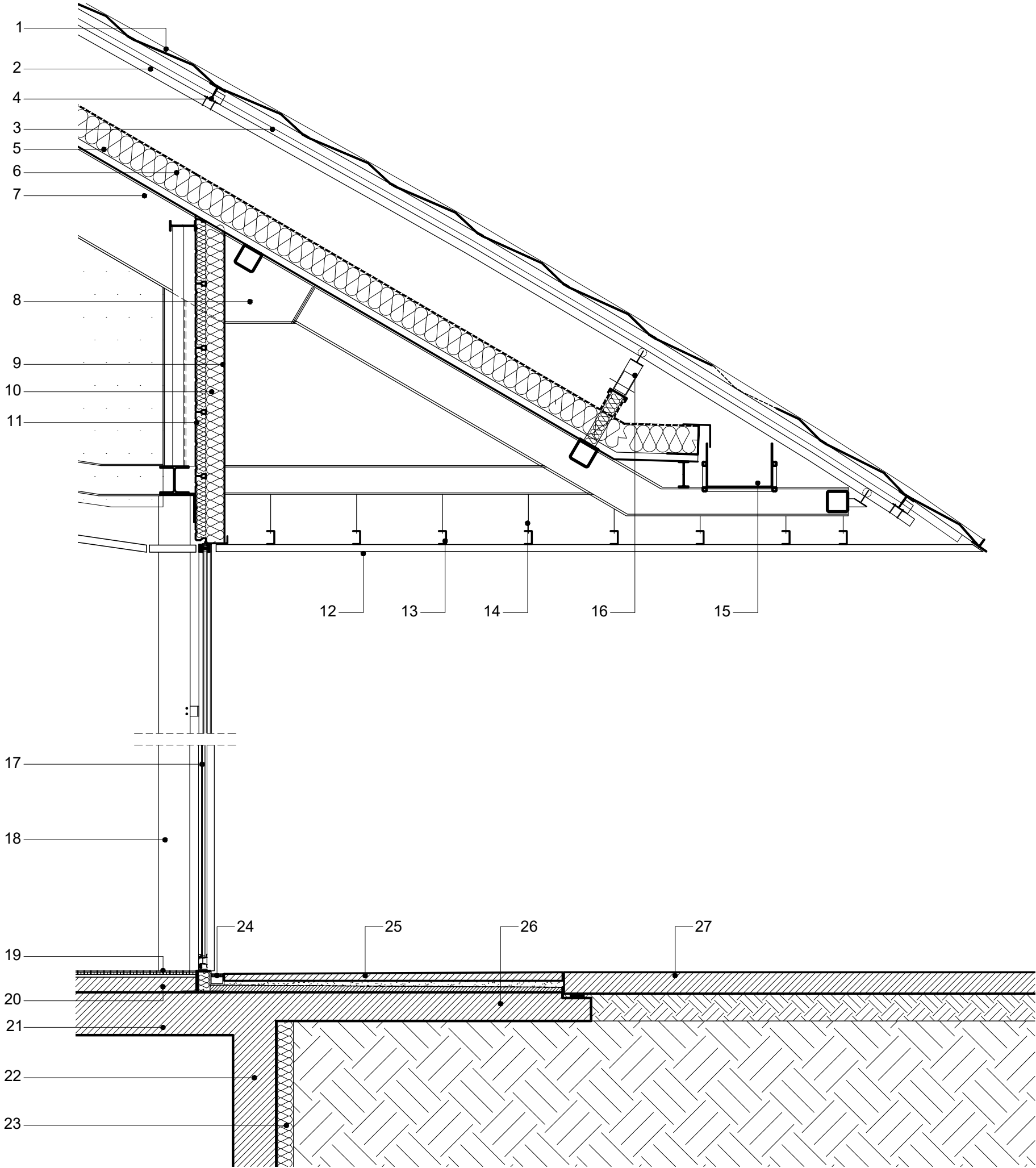
Detailed section, lobby façade and roof
