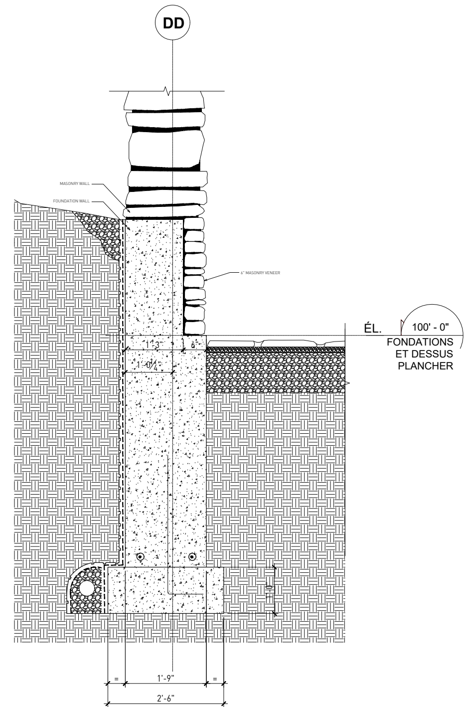
Landscape stone wall
