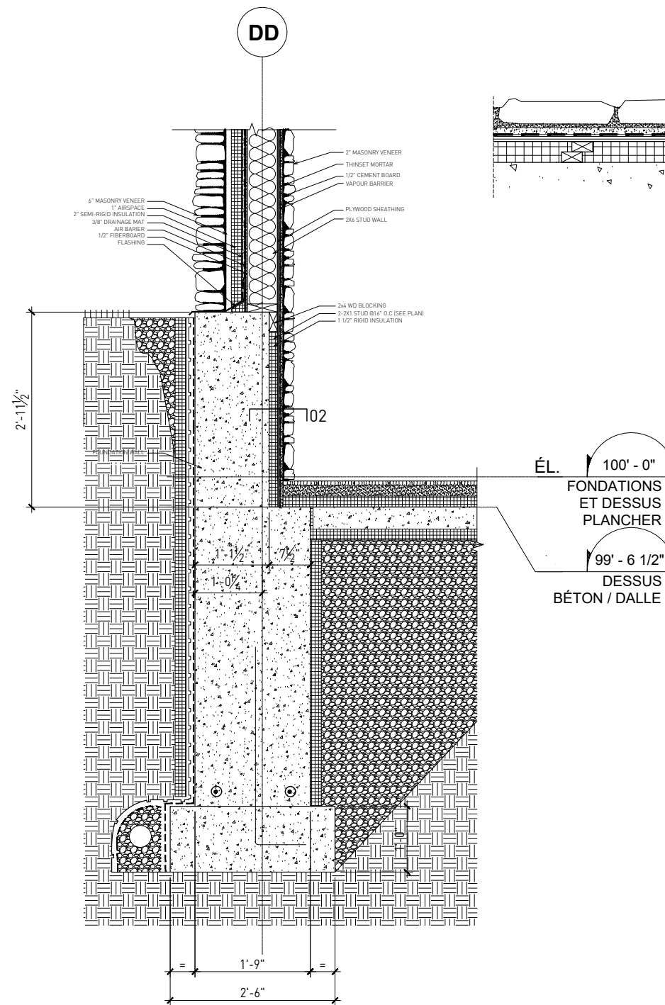
Stud wall with insulation and exterior and interior stone veneer
