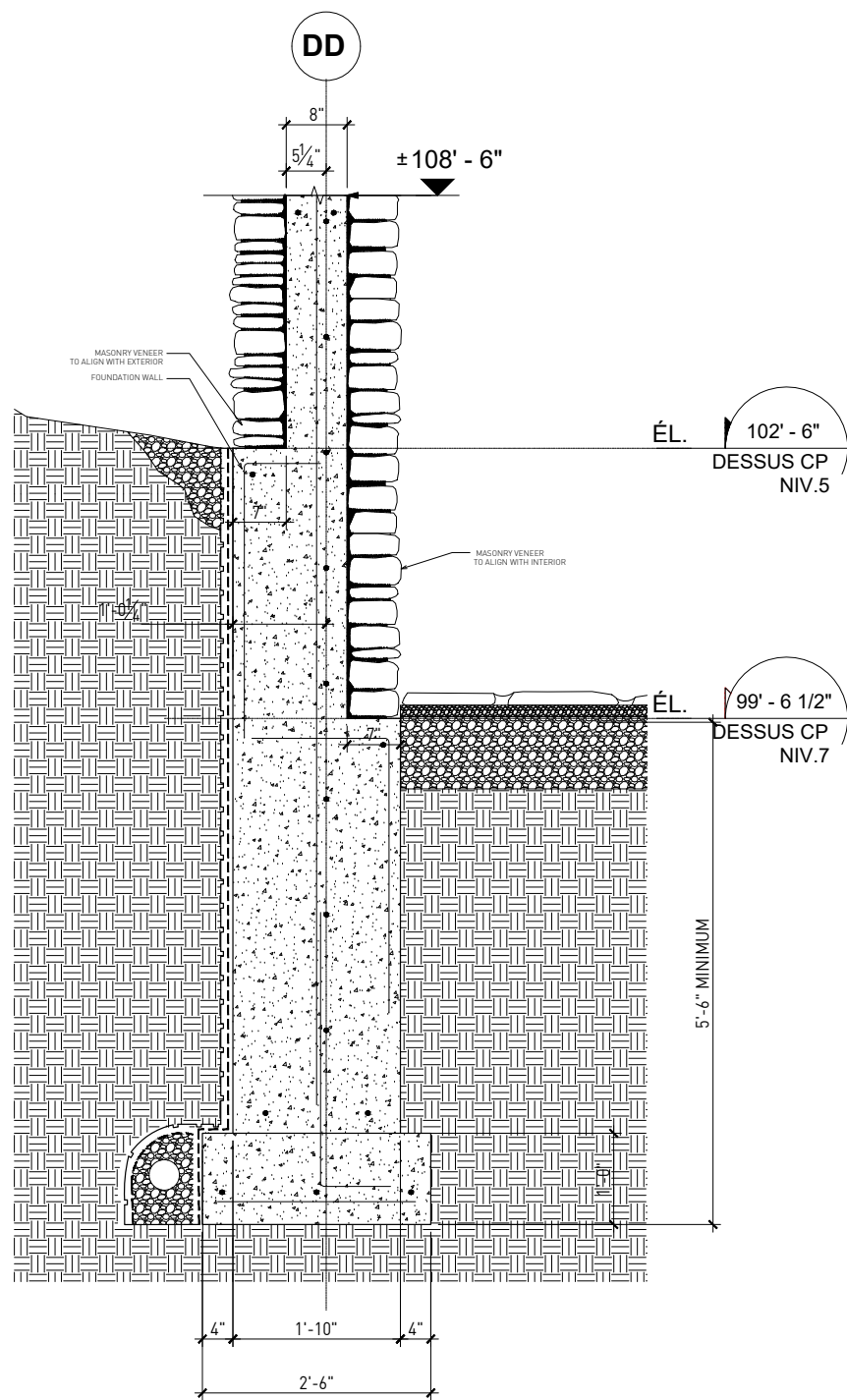
Concrete wall with stone veneer
