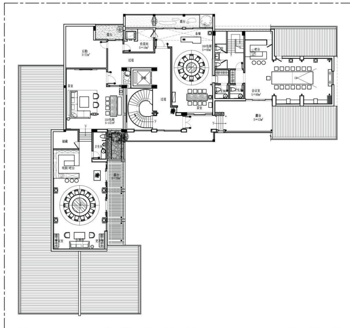
Third floor
