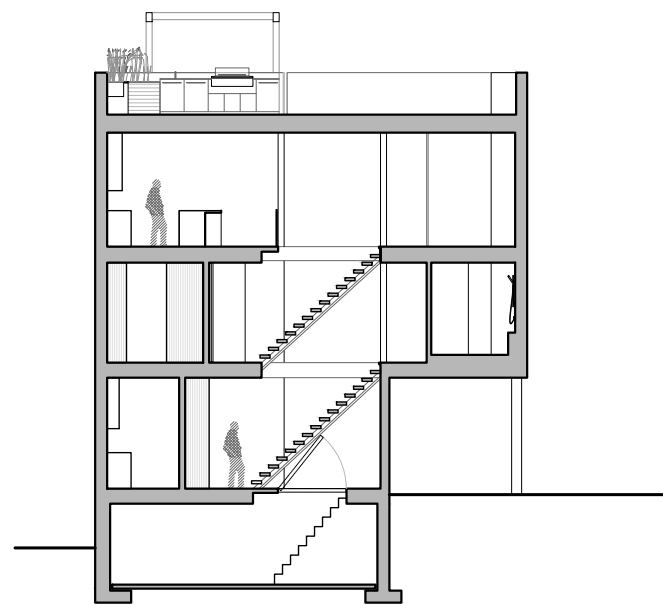
SECTION 2 0' 5' 20'
