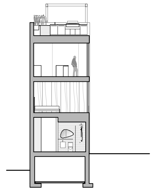
SECTION 3 0' 5' 20'
