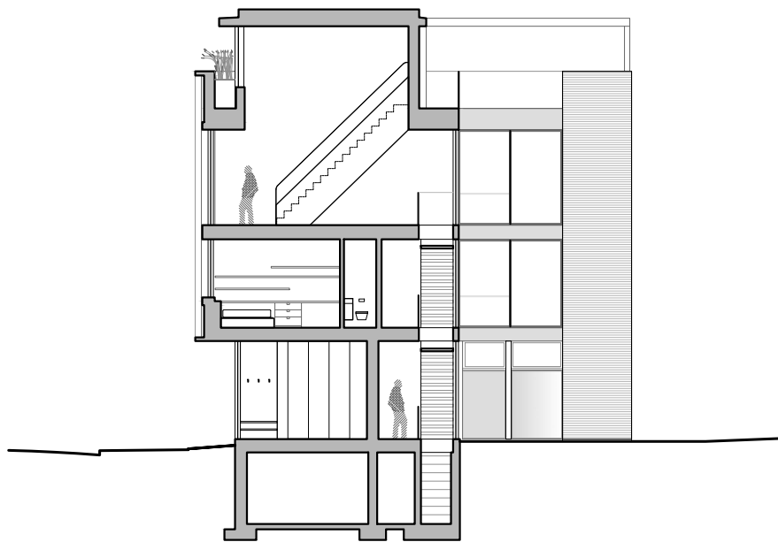
SECTION A 0' 5' 20'
