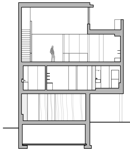
SECTION 1 0' 5' 20'
