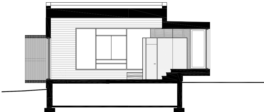
SECTION 2 scale : \frac{3}{32}'' = 1'-0''
