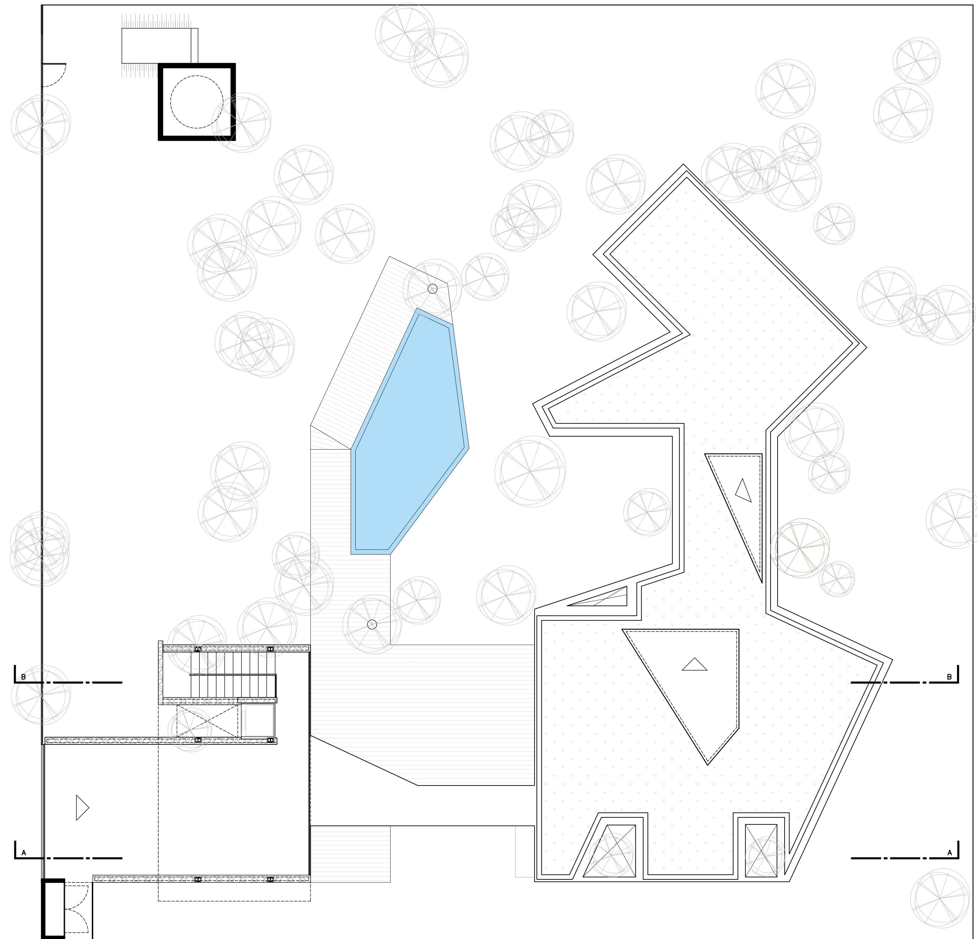
3RD FLOOR PLAN
