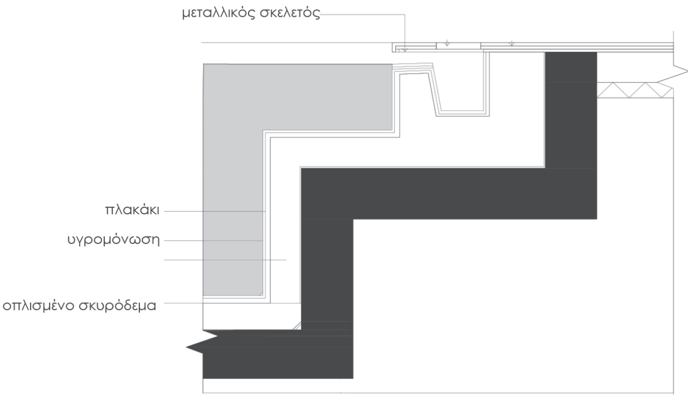
Swimming pool construction detail
