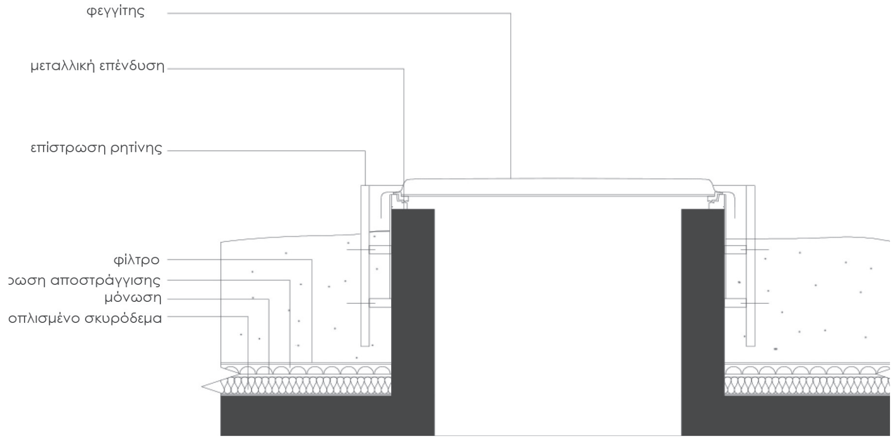
Skydome construction detail
