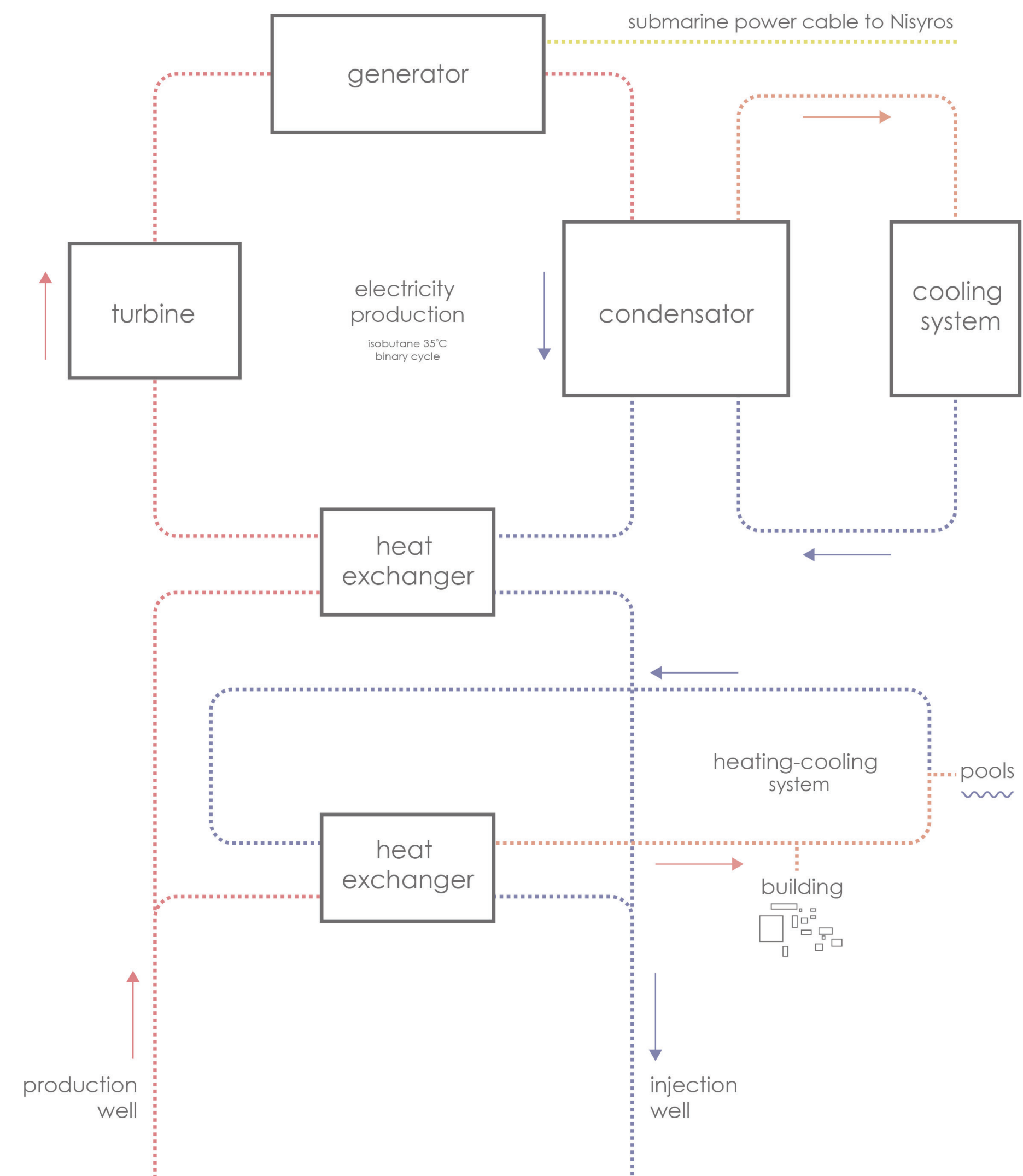
Binary cycle power plant
