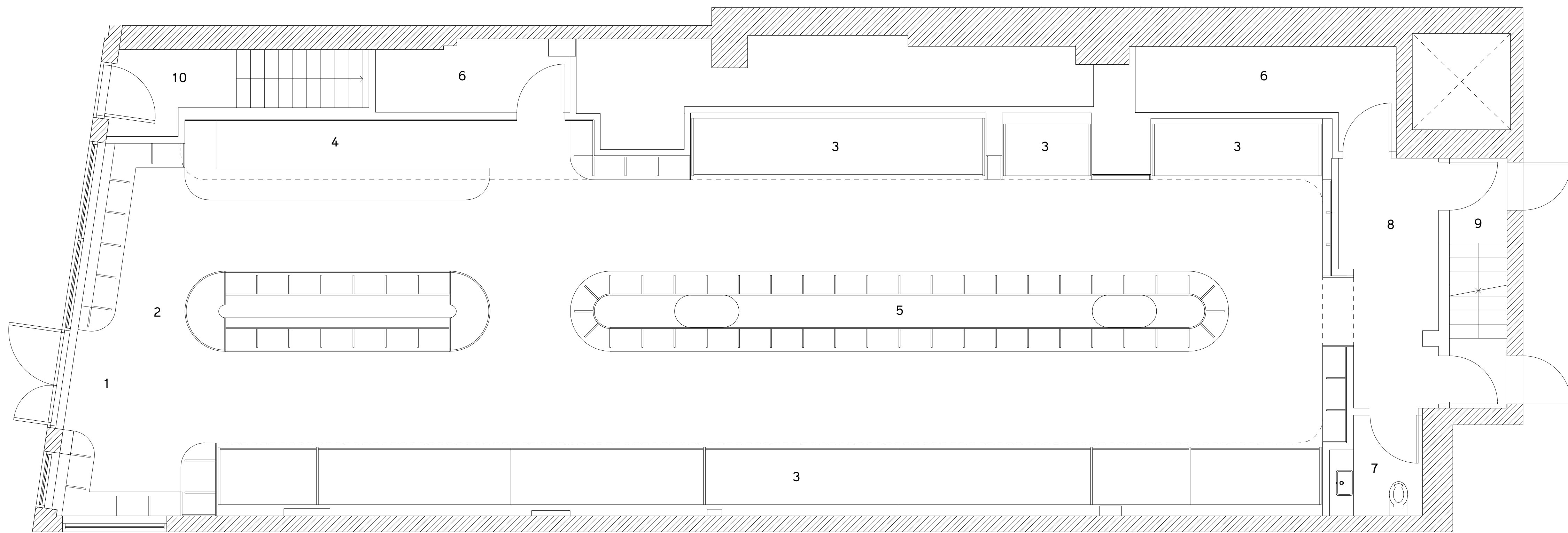
Floor Plan
