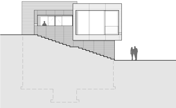
Élévation sud South Elevation
