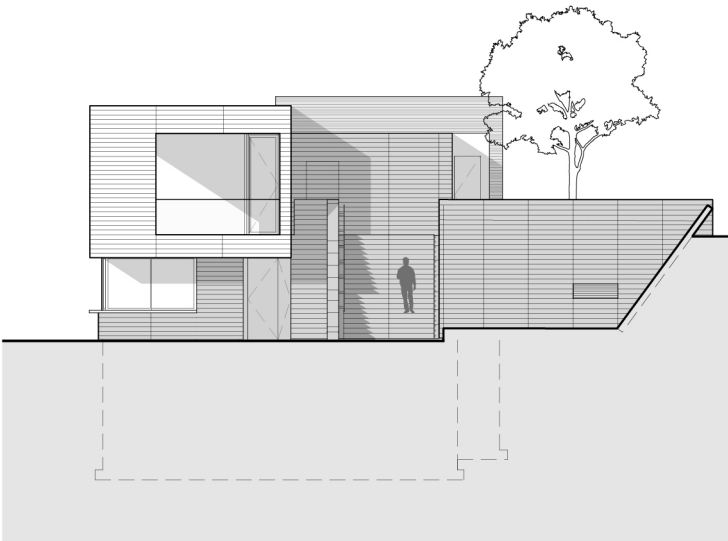
Élévation nord North Elevation
