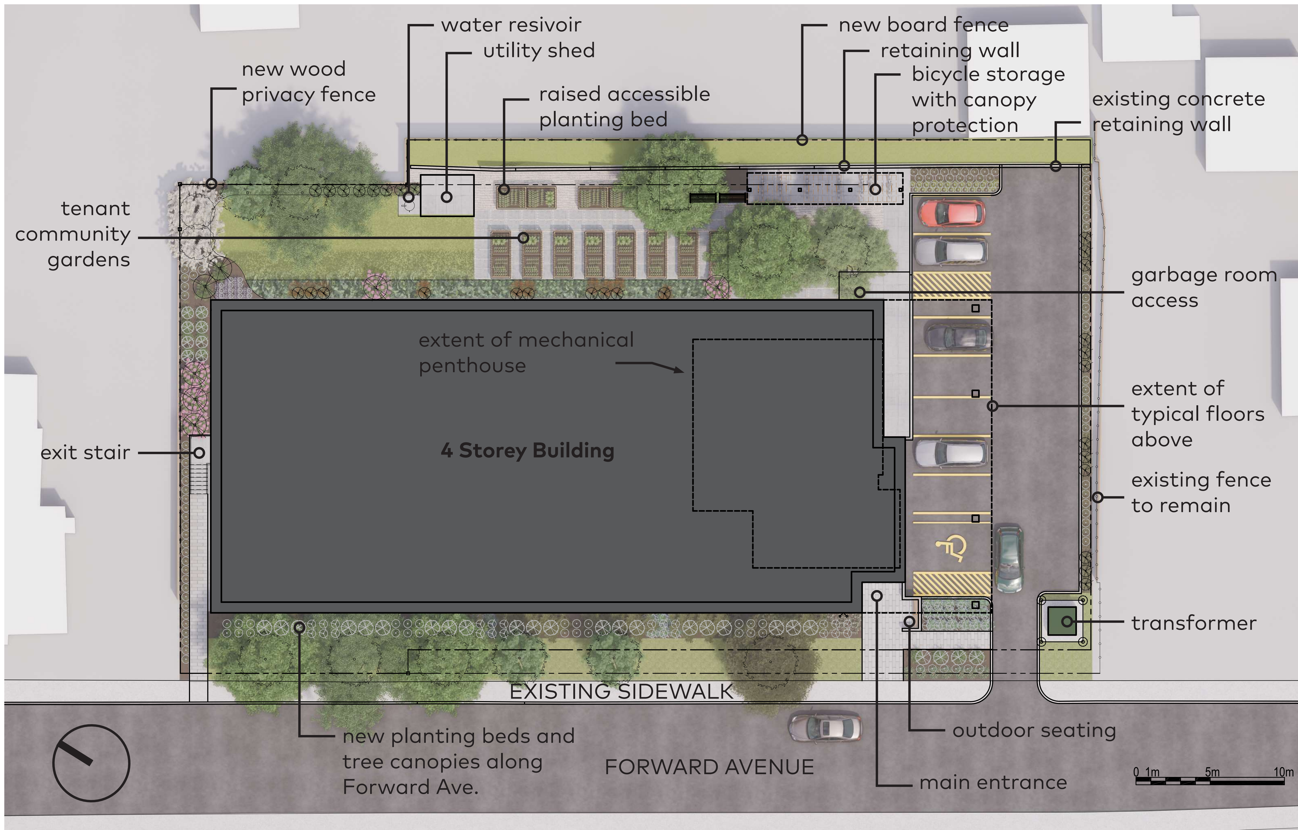
Site Plan - 159 Forward Ave
