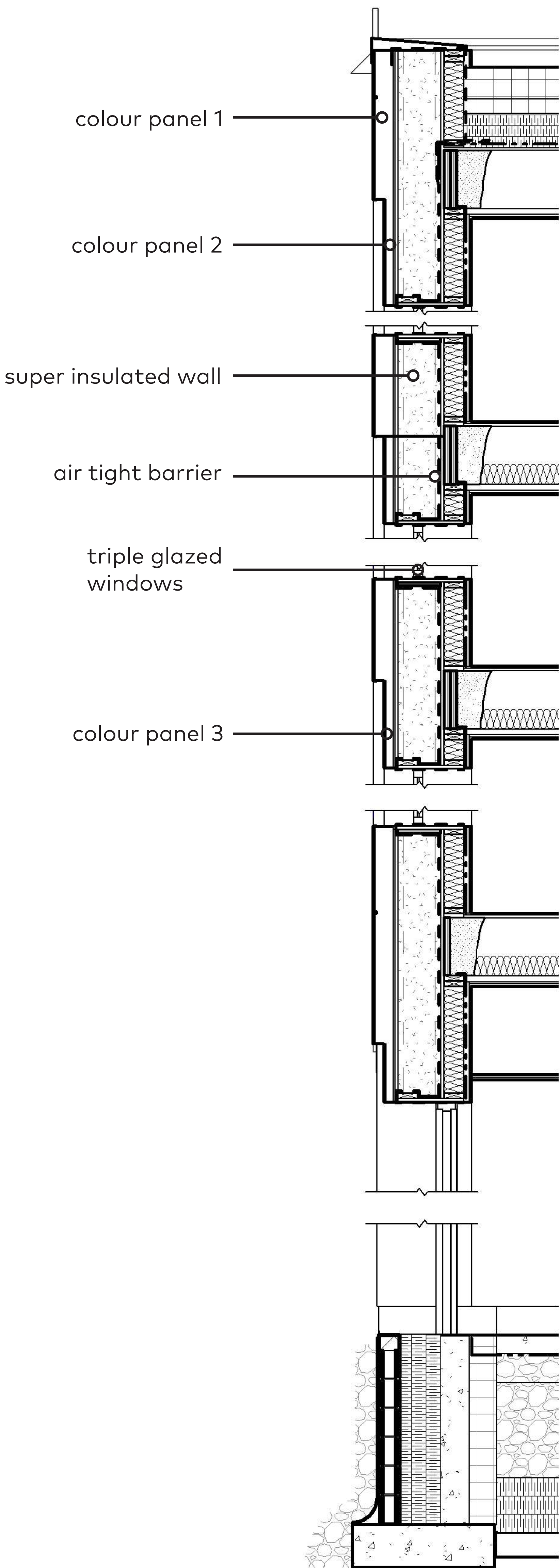
Wall Section (1:50)
