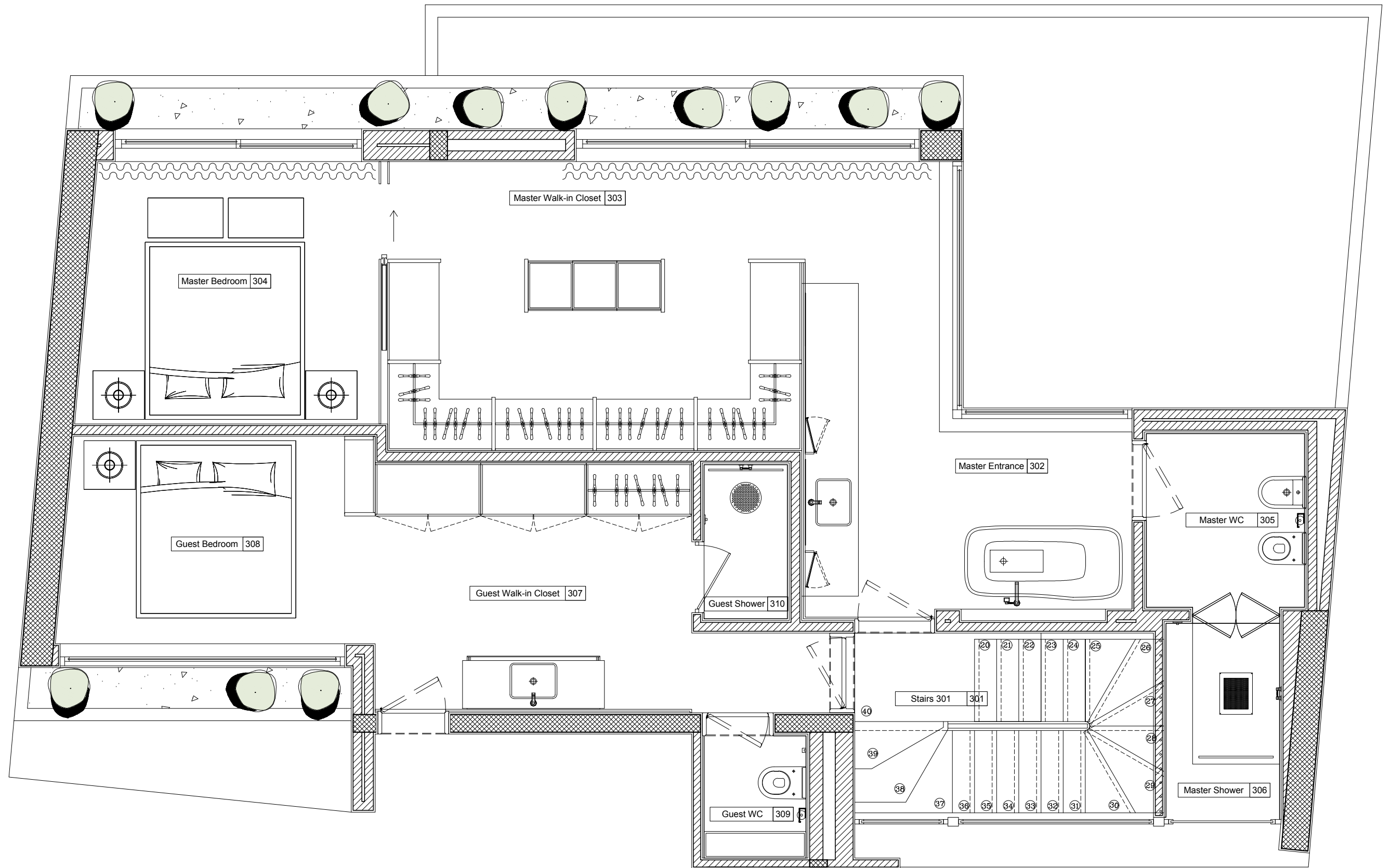
AD 165 - MALLORCA TRIPLEX - 13TH FLOOR
