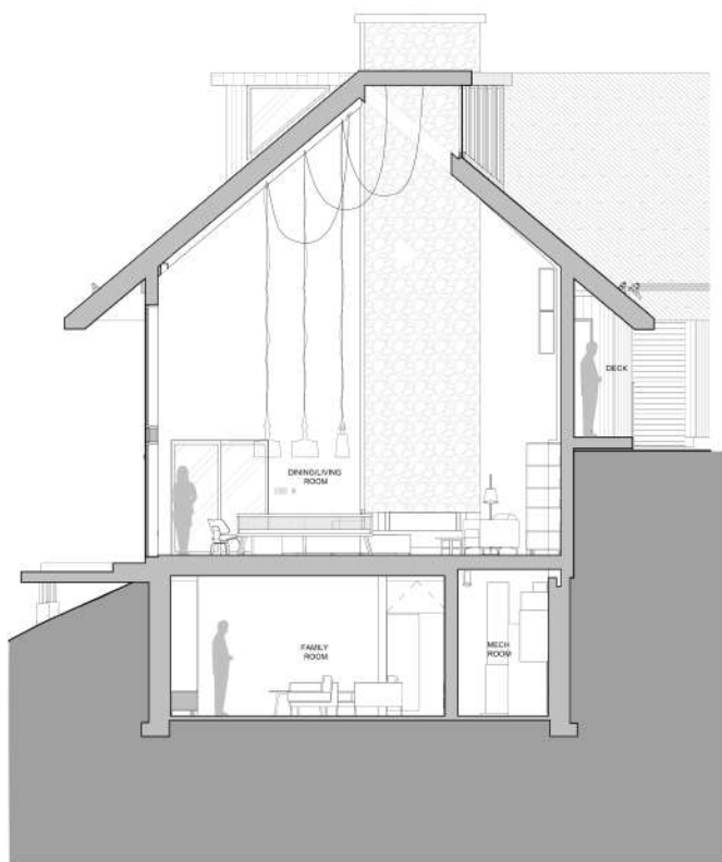
CROSS SECTION - LIVING ROOM
