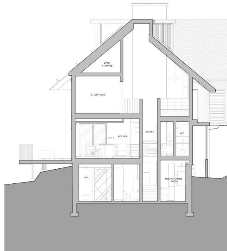
CROSS SECTION - KITCHEN
