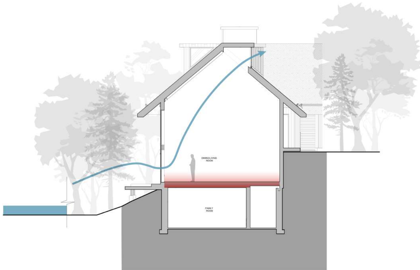
CROSS SECTION - LIVING ROOM
