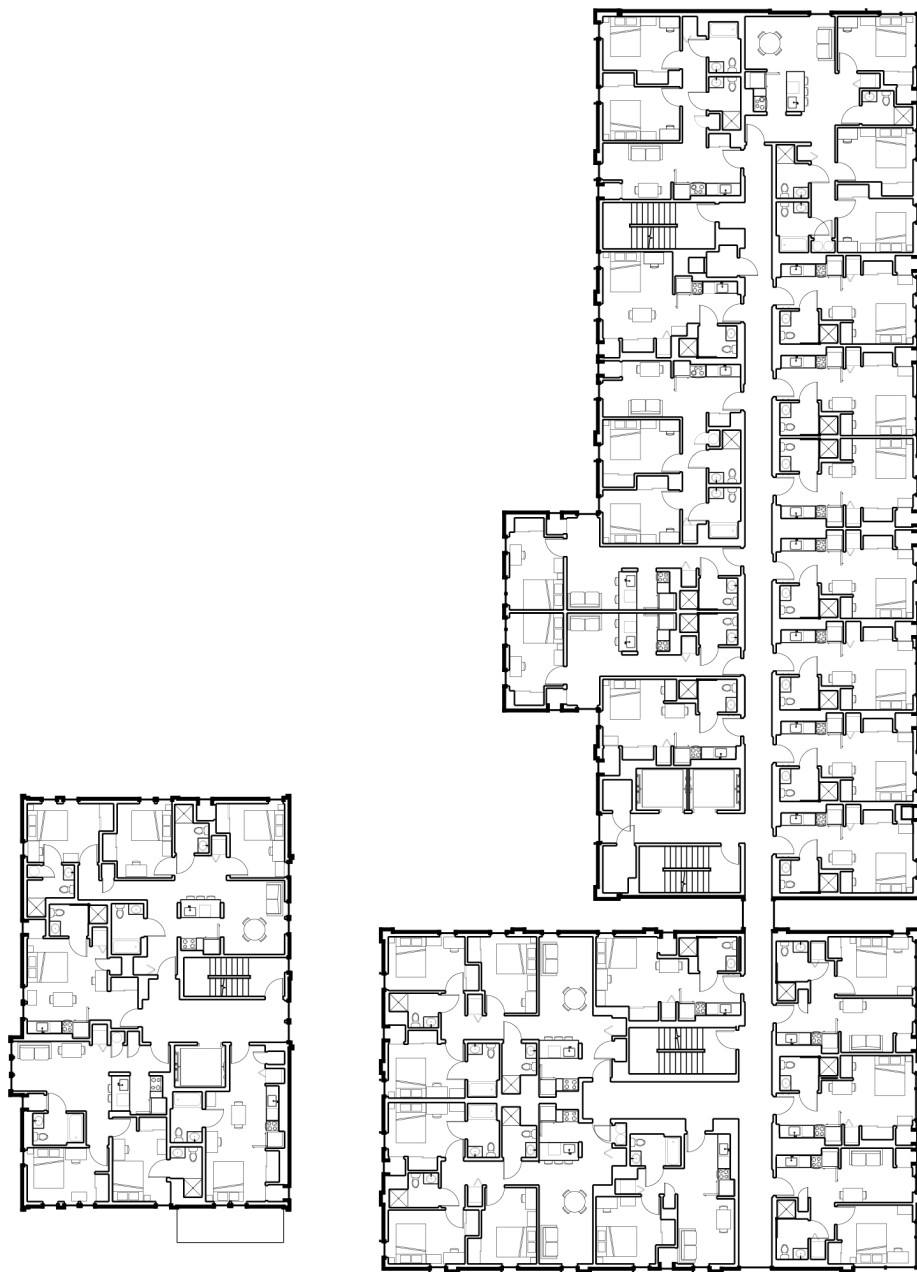
Catherine South Residential Floor Plan
