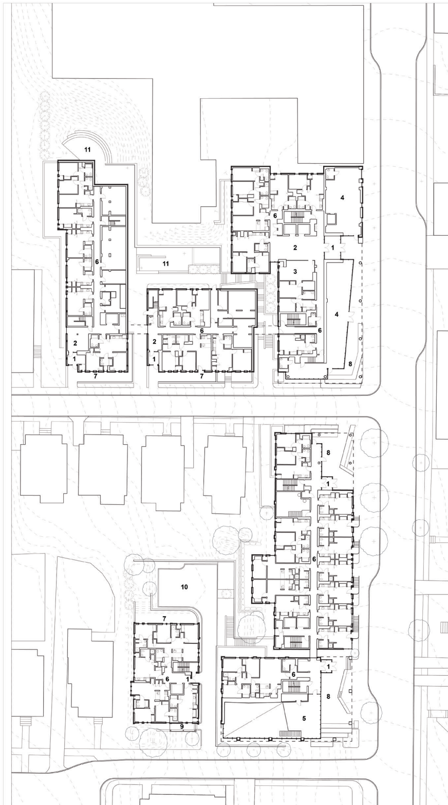
Catherine Commons Ground Floor Plan
