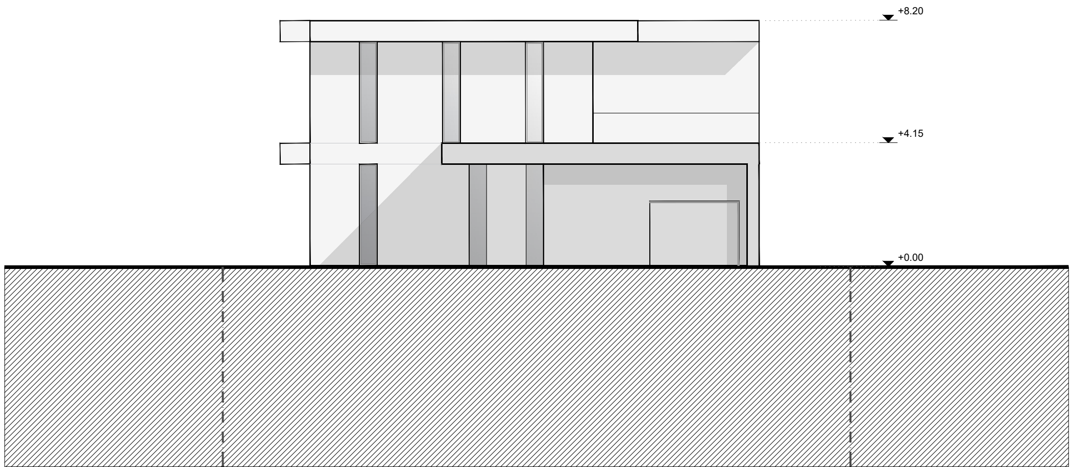
NORTH ELEVATION
