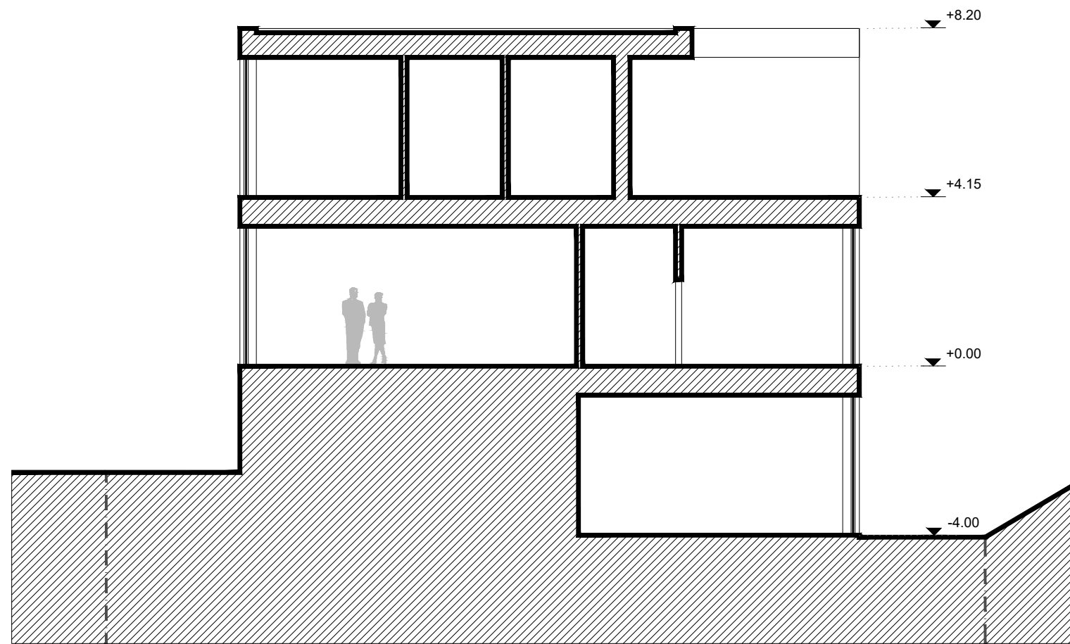
SECTION B-B
