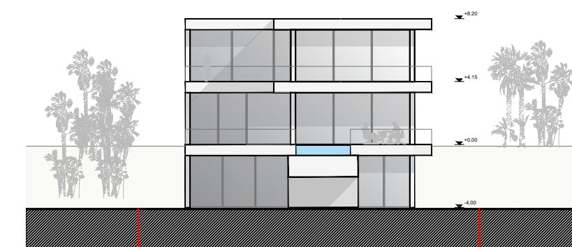
SOUTH ELEVATION
