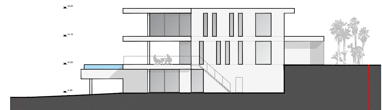
EAST ELEVATION
