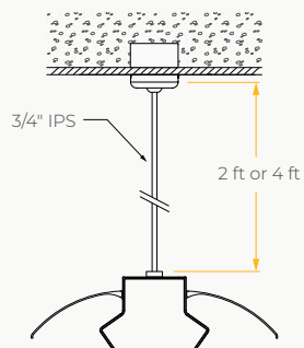
Stem Mount
