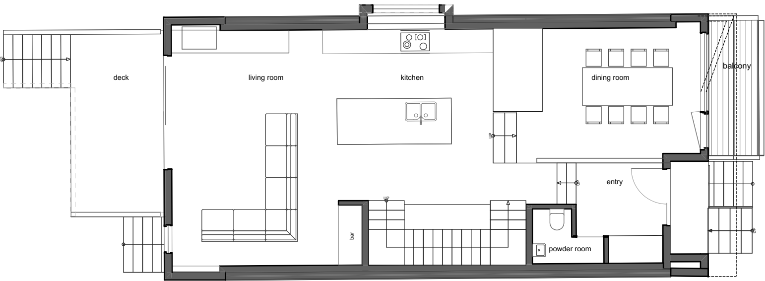
Main Floor
