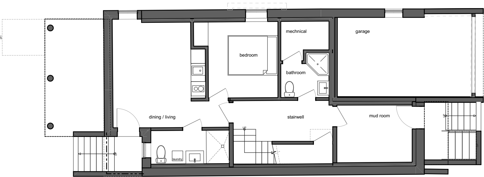
Lower Level
