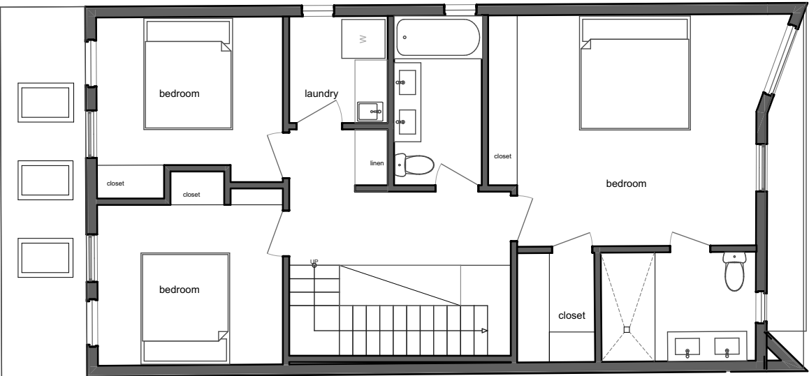
2nd Floor
