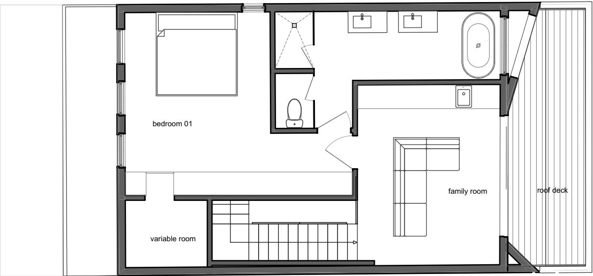
3rd Floor
