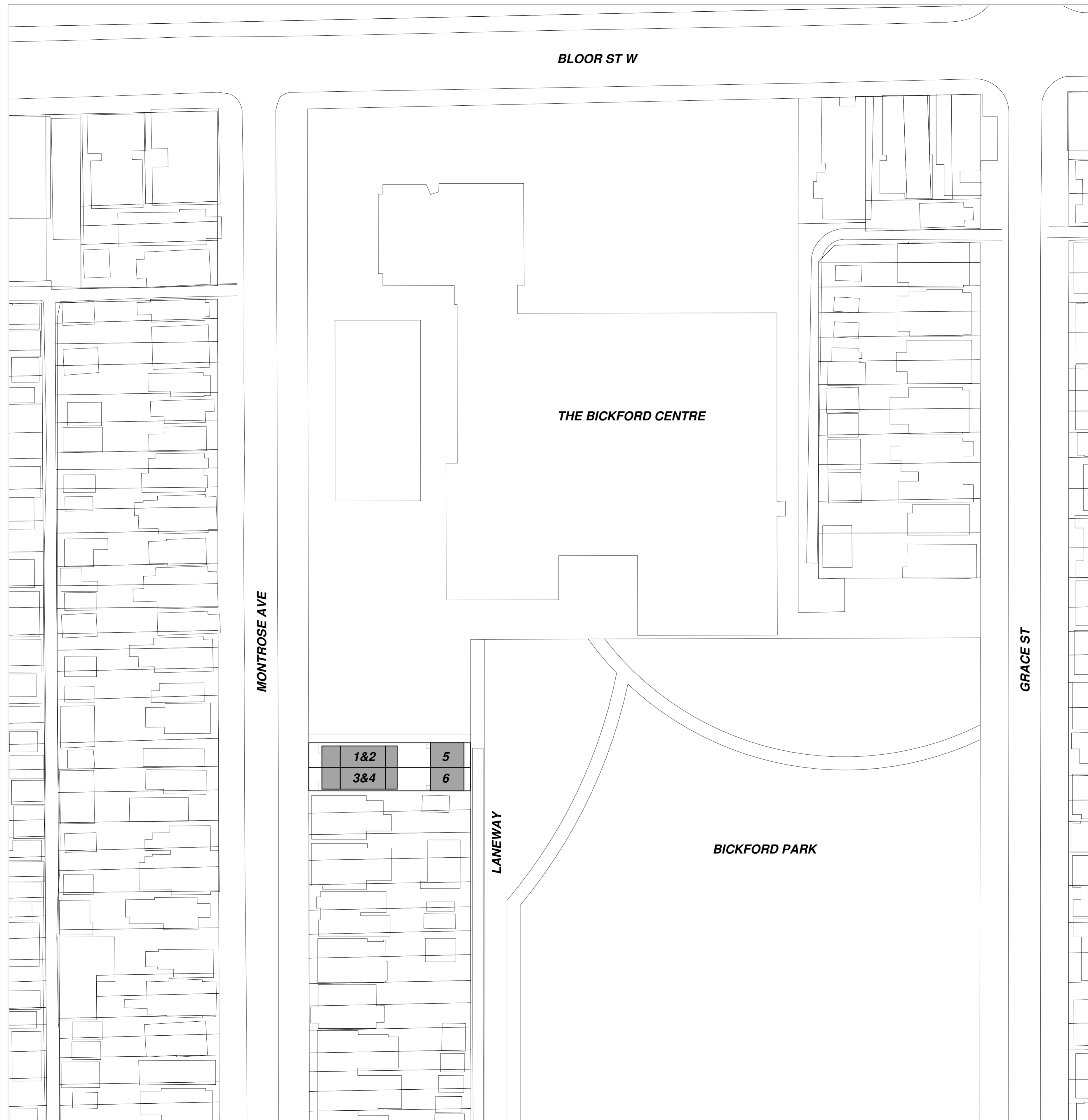
SITE PLAN
