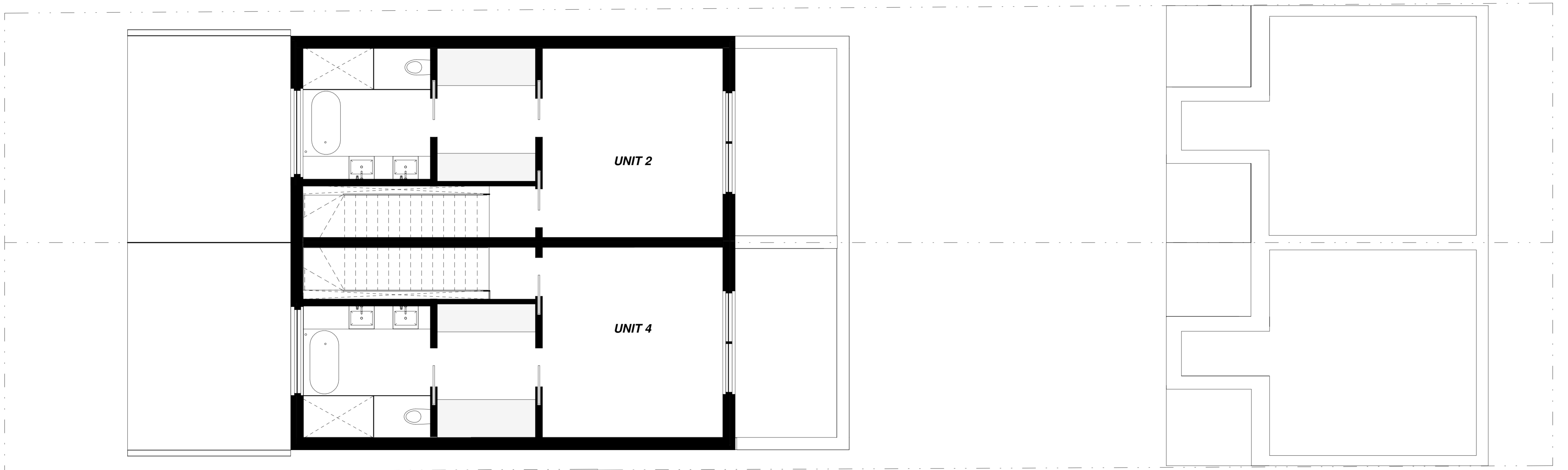
THIRD LEVEL
