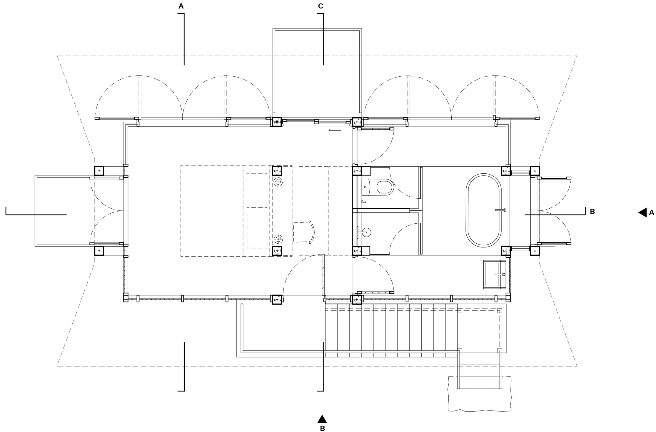
Hotel Room 2F Plan
