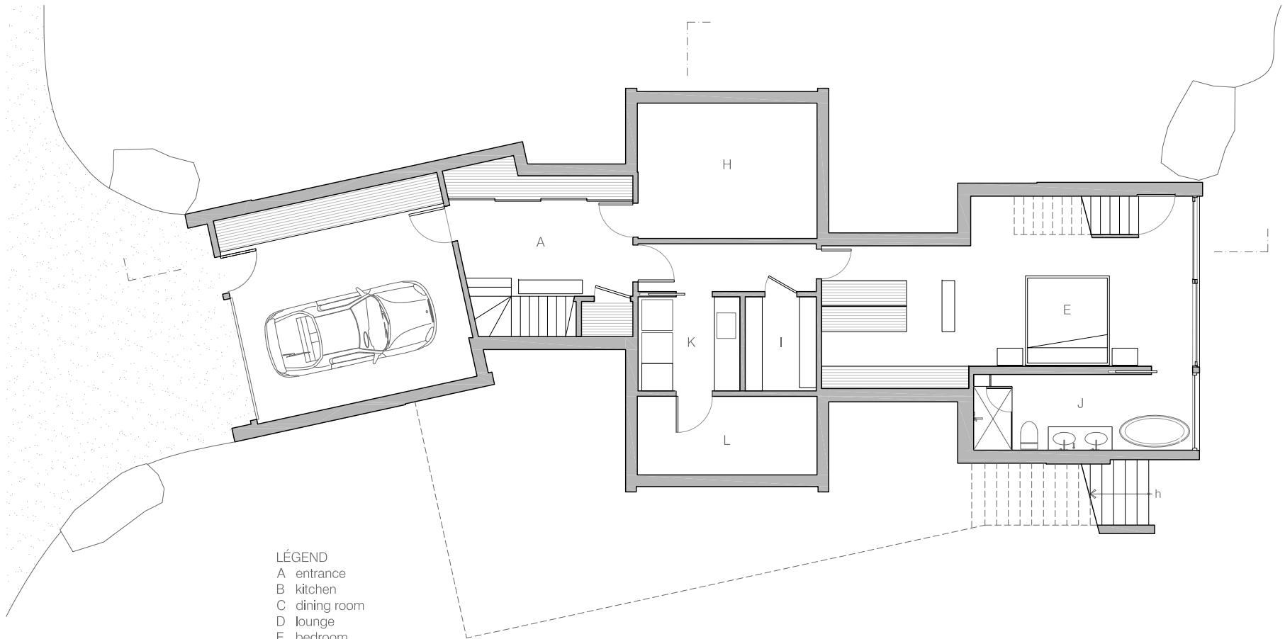
BASEMENT/ GROUND FLOOR PLAN
