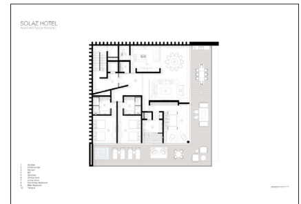
2018_Solaz_Los_Cabos_SMA_PLANS_Apartment_Typical.jpg Image Description: Apartment Typical Floorplan Image Credit: © Sordo Madaleno Arquitectos, english and spanish version
