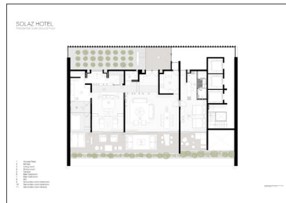
2018_Solaz_Los_Cabos_SMA_PLANS_Presidential_Suite.jpg Image Description: Presidential Suite Image Credit: © Sordo Madaleno Arquitectos, english and spanish version
