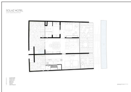
2018_Solaz_Los_Cabos_SMA_PLANS_Jr_Suite.jpg Image Description: Jr Suite Image Credit: © Sordo Madaleno Arquitectos, english and spanish version
