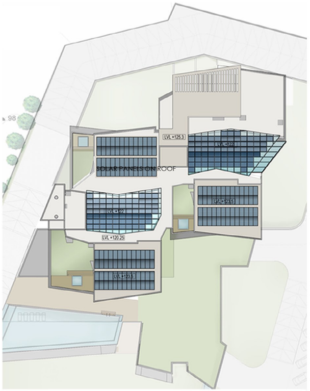
TERRACE PLAN
