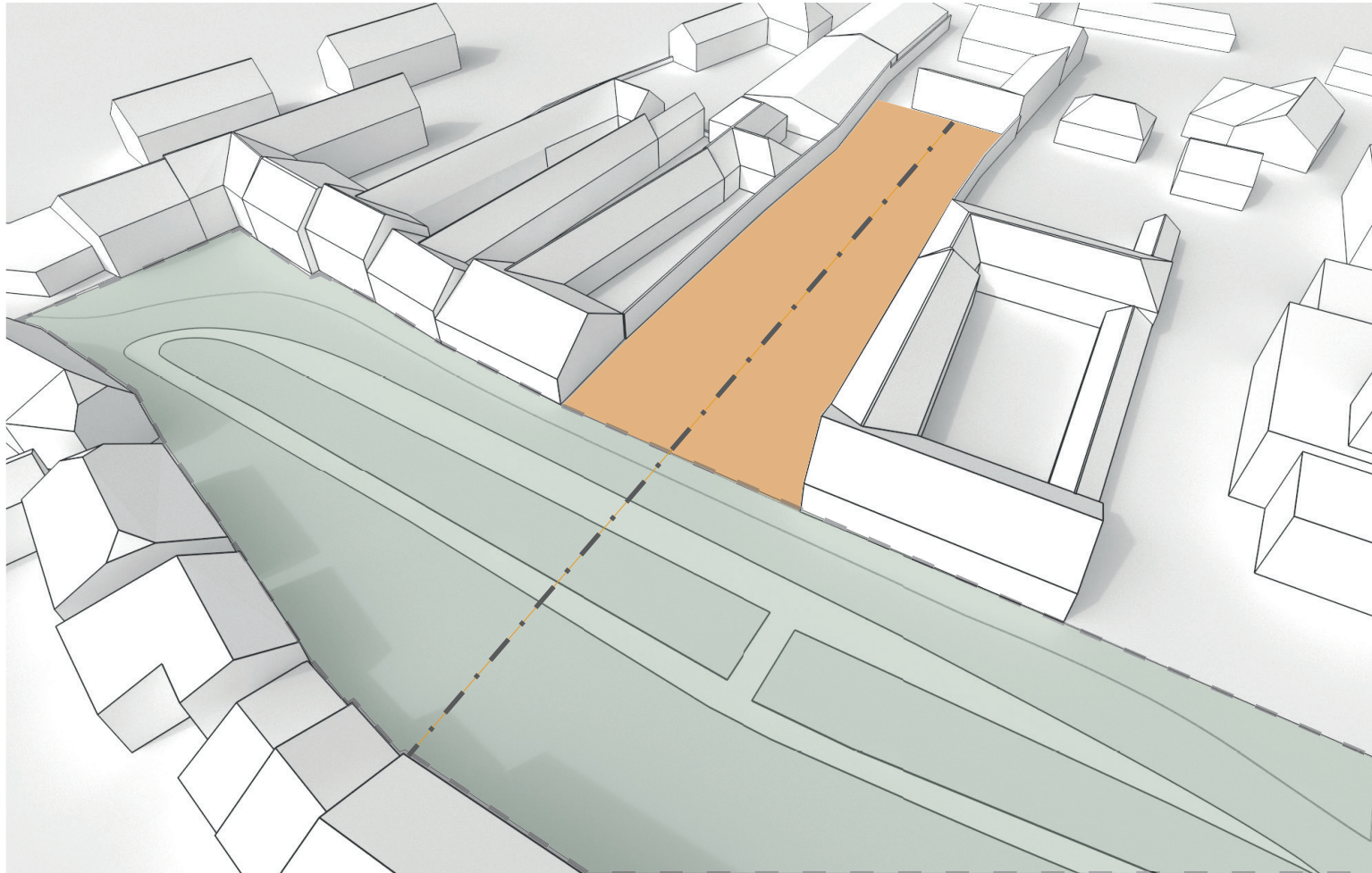
STRONG SYMMETRY
