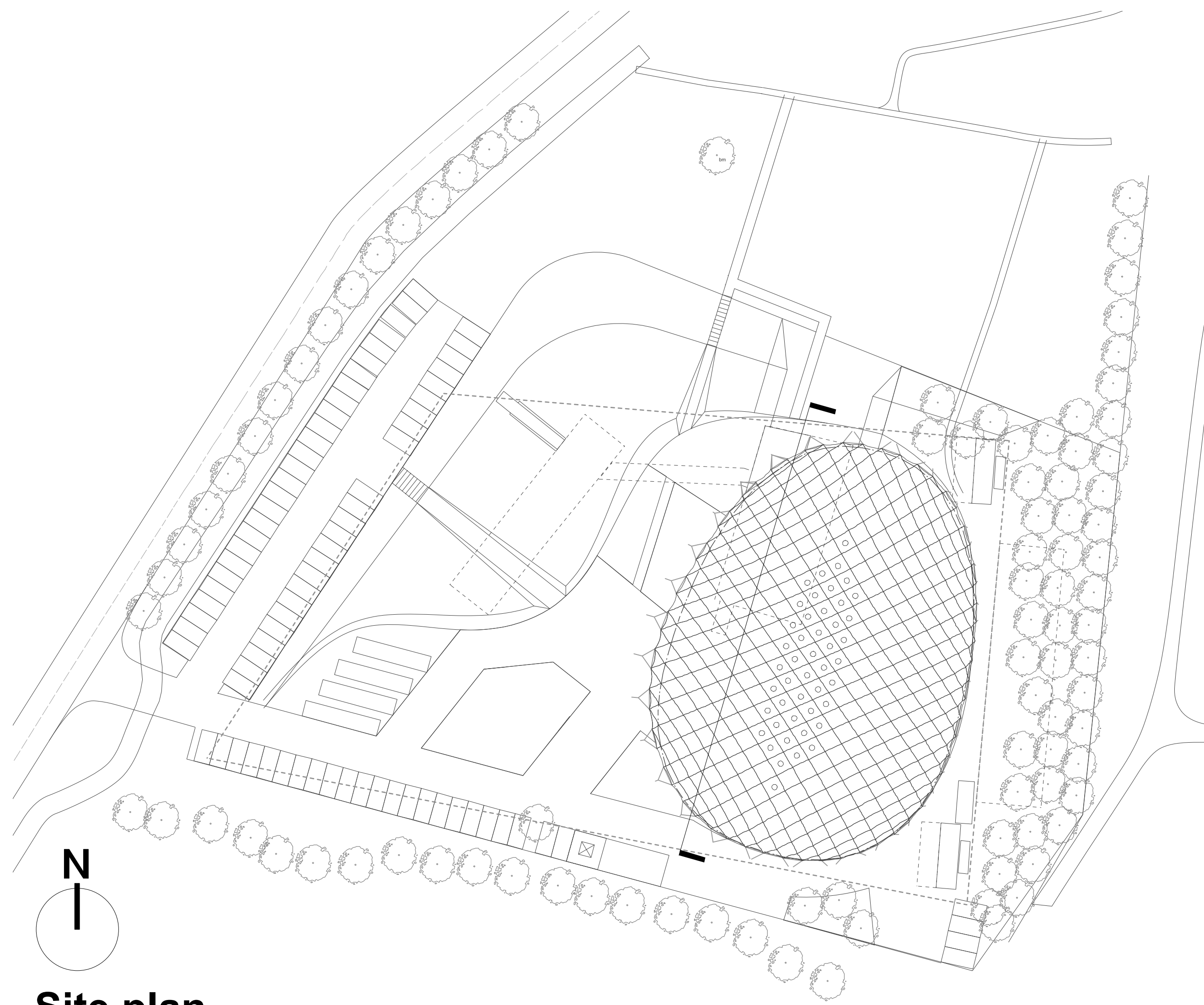
Site plan
