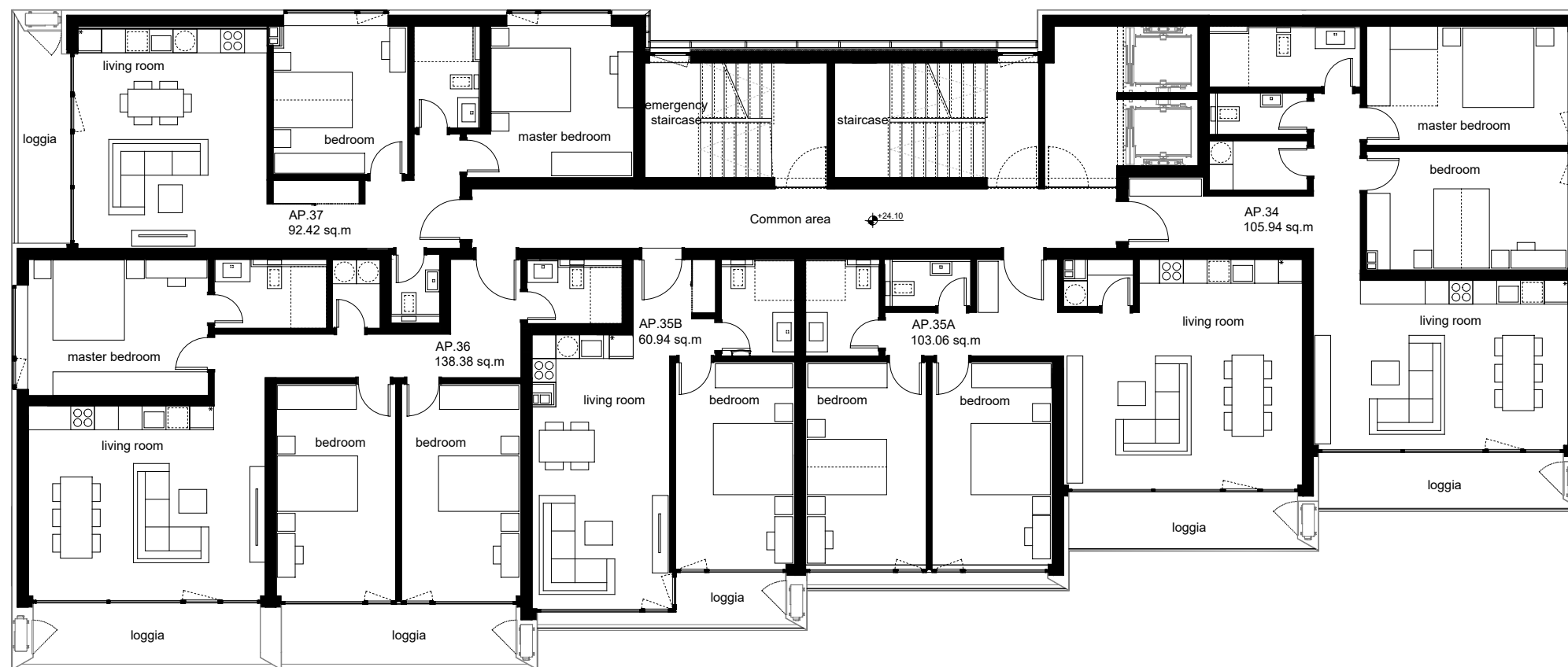
Floor Plan 9th Floor 0m 1m 2m 5m
