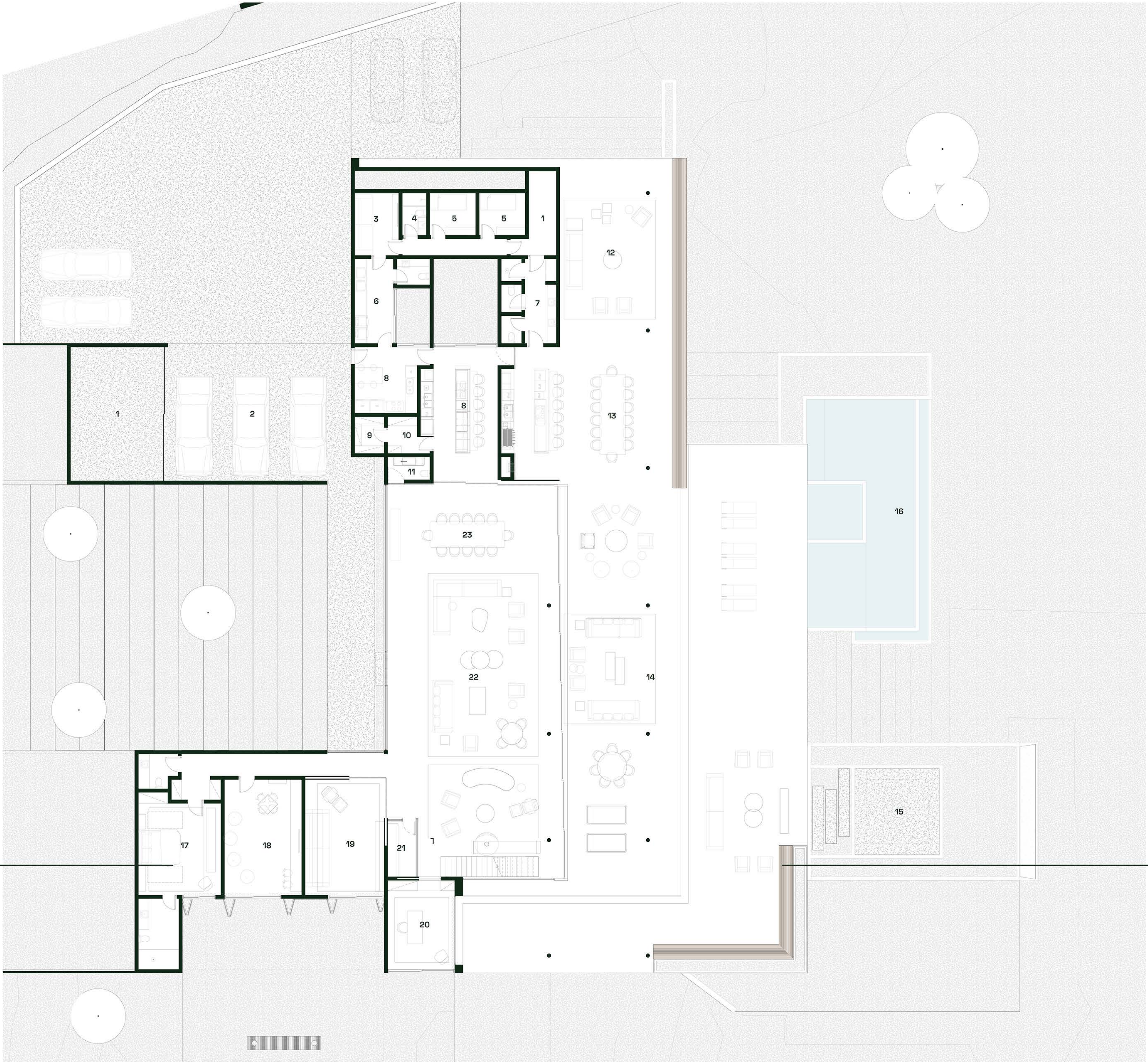
PLANTA PAVIMENTO TÉRREO | GROUND FLOOR PLAN
