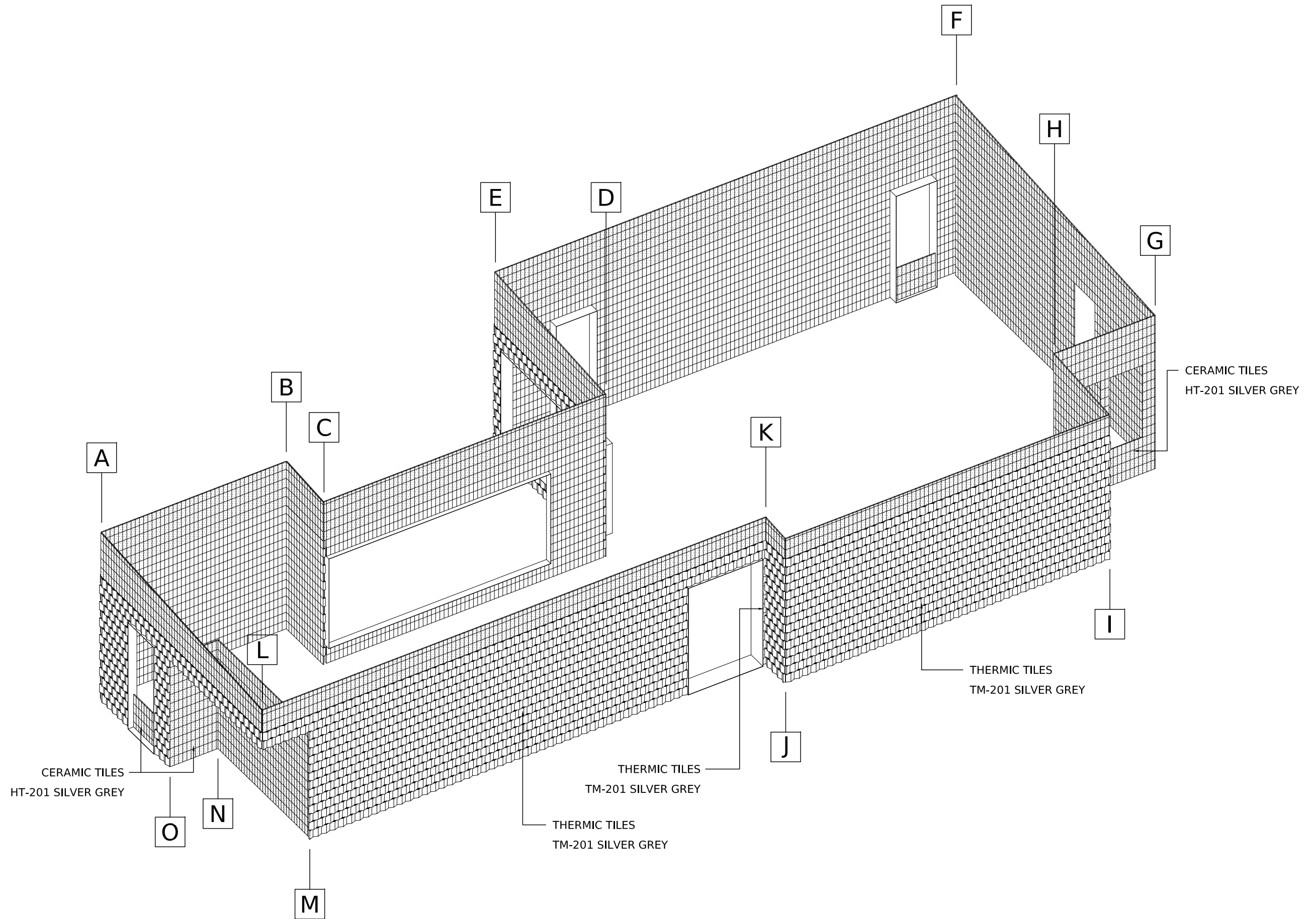
KEY ISOMETRIC FOR INSTALLATION OF THERMIC TILES
