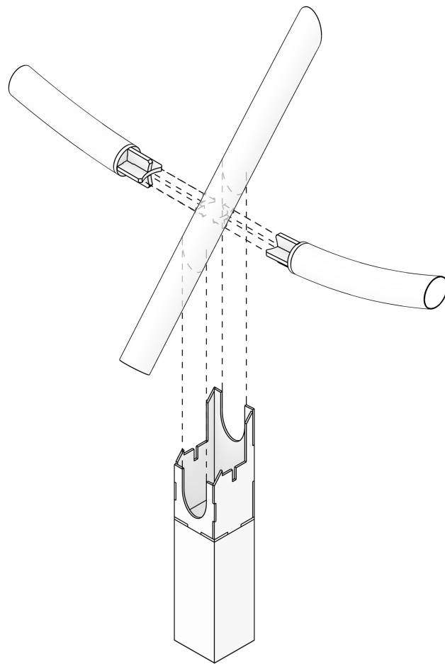
Connecting Plates
