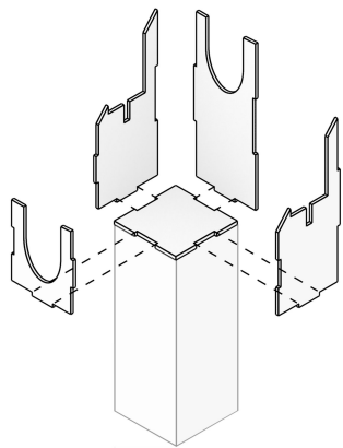
Junction Box
