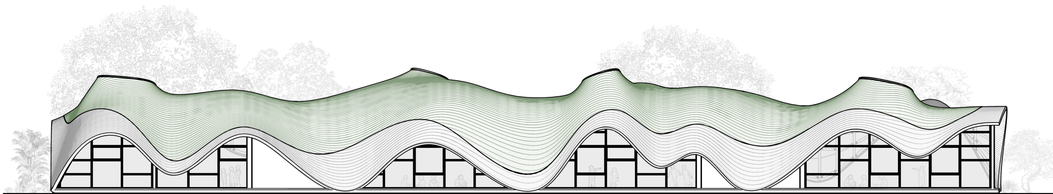
South Elevation
