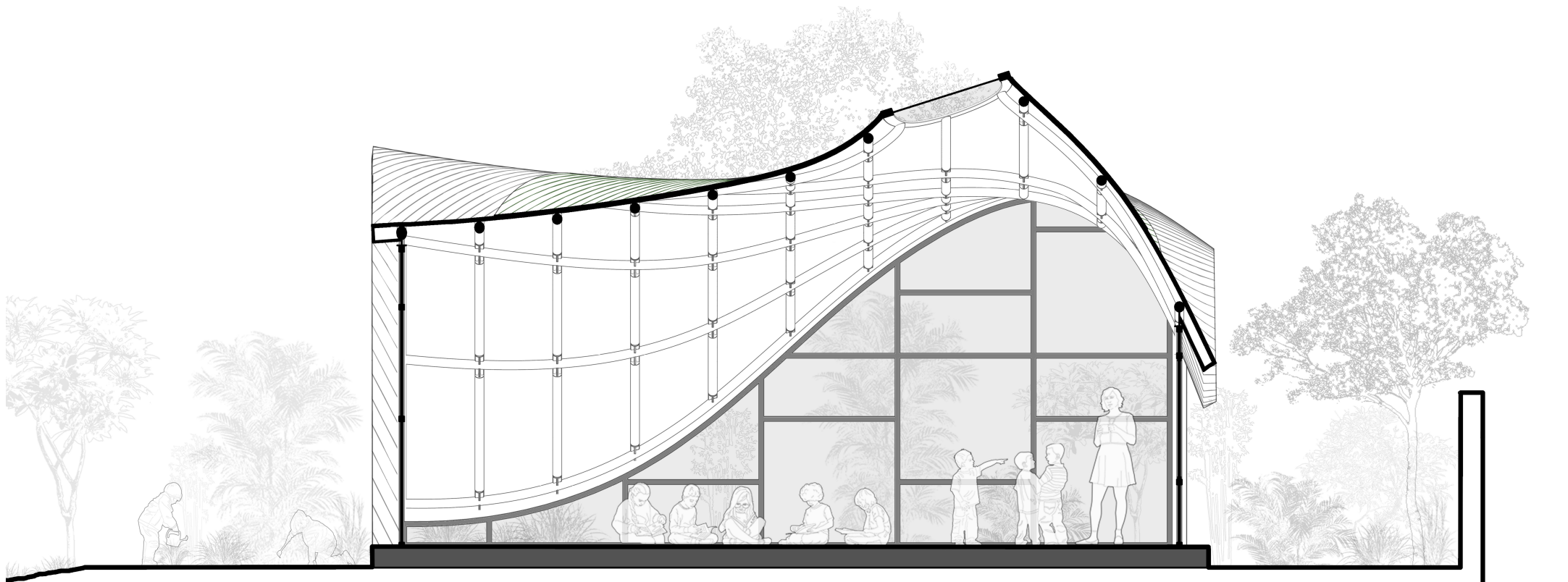
Transverse Section
