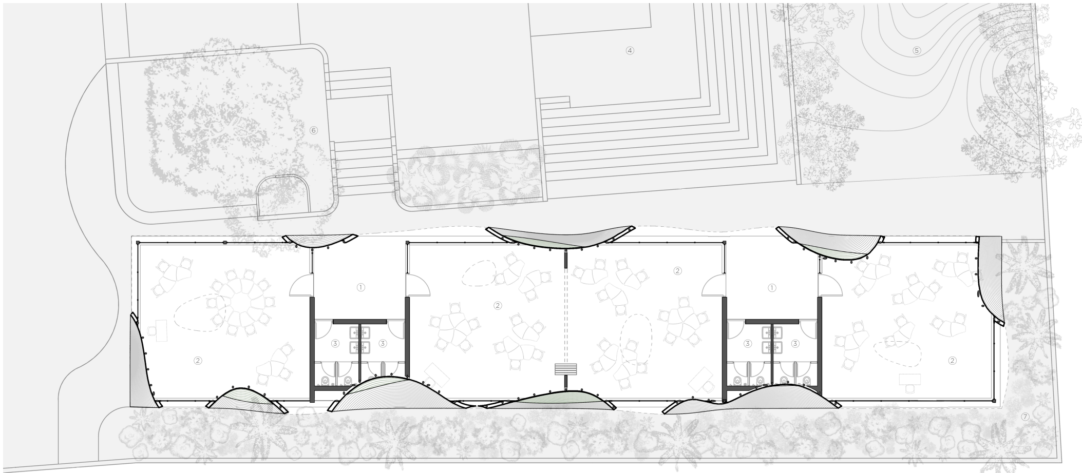
Layout Plan
