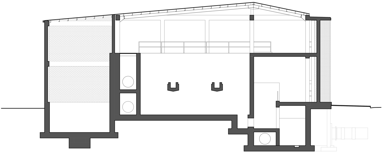
SECTION BB
