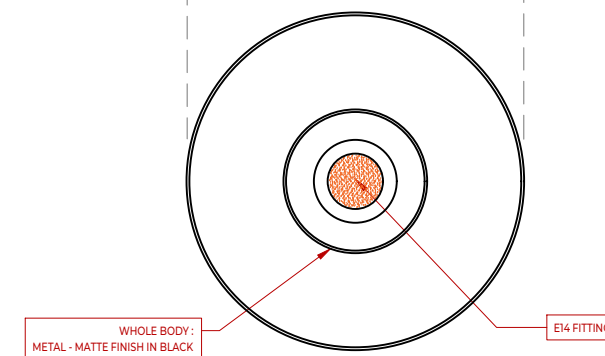
PLATFORM DETAIL
