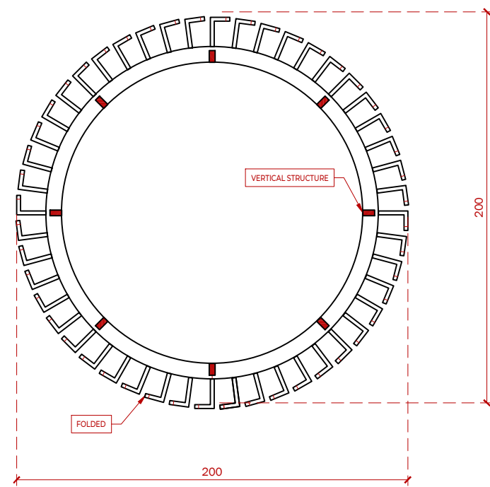
RING DETAIL
