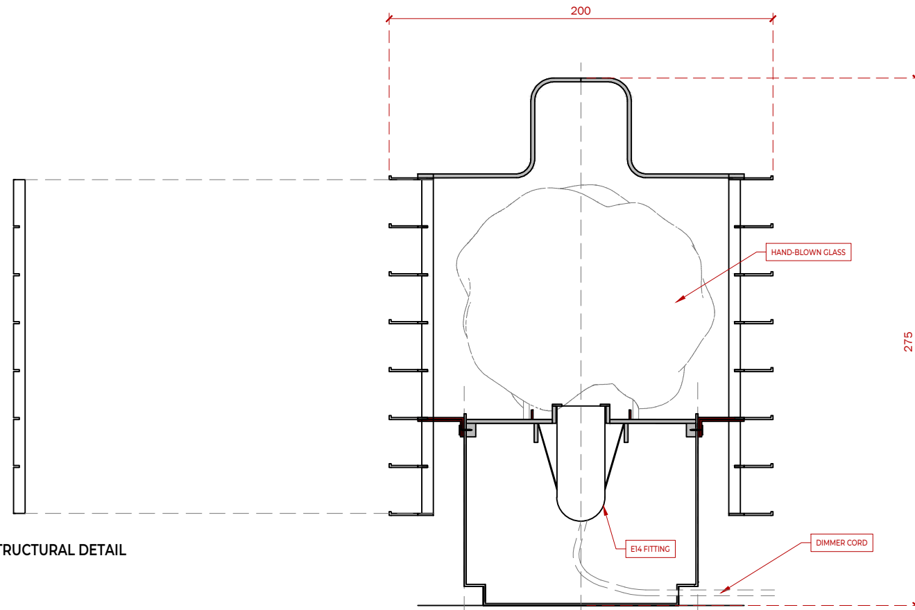
SECTION DETAIL
