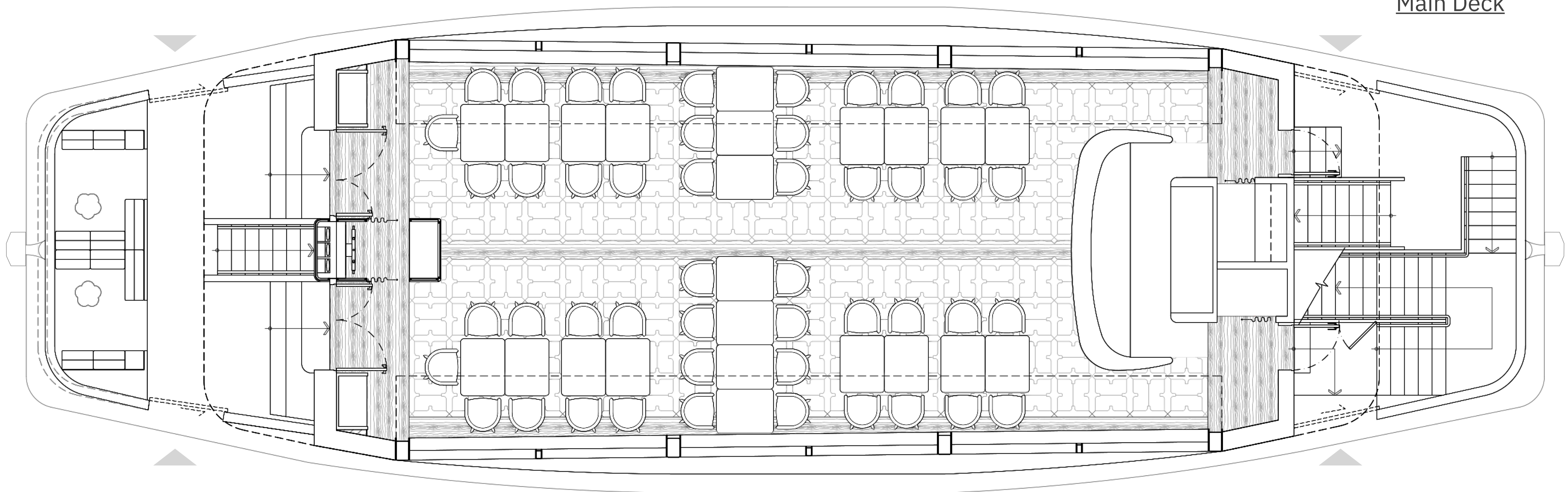
Main Deck
