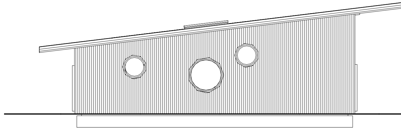
PR1 & 2 North Elevation Scale: 1:100
