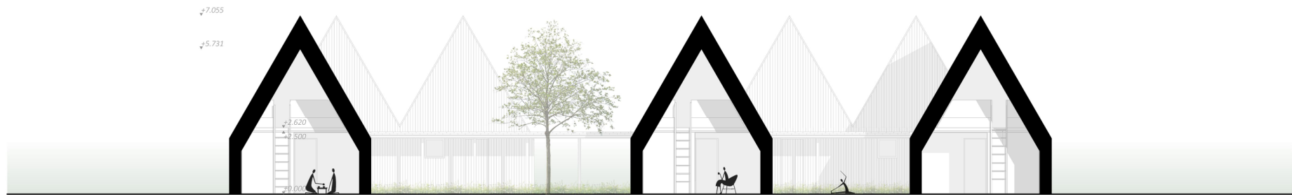
HERB VILLAS - SECTION 1-1
