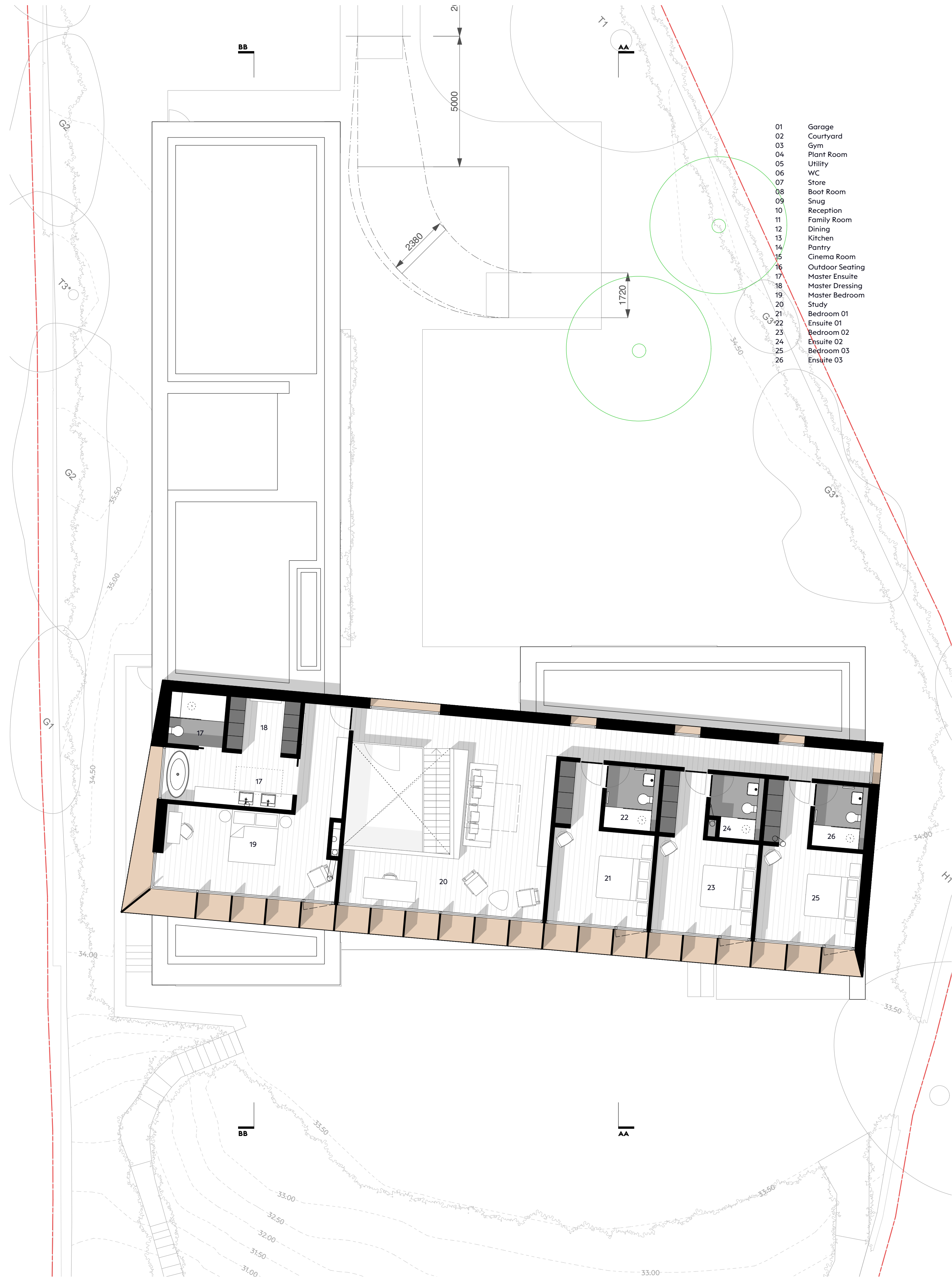
FIRST FLOOR PLAN 1:100 @ A1
