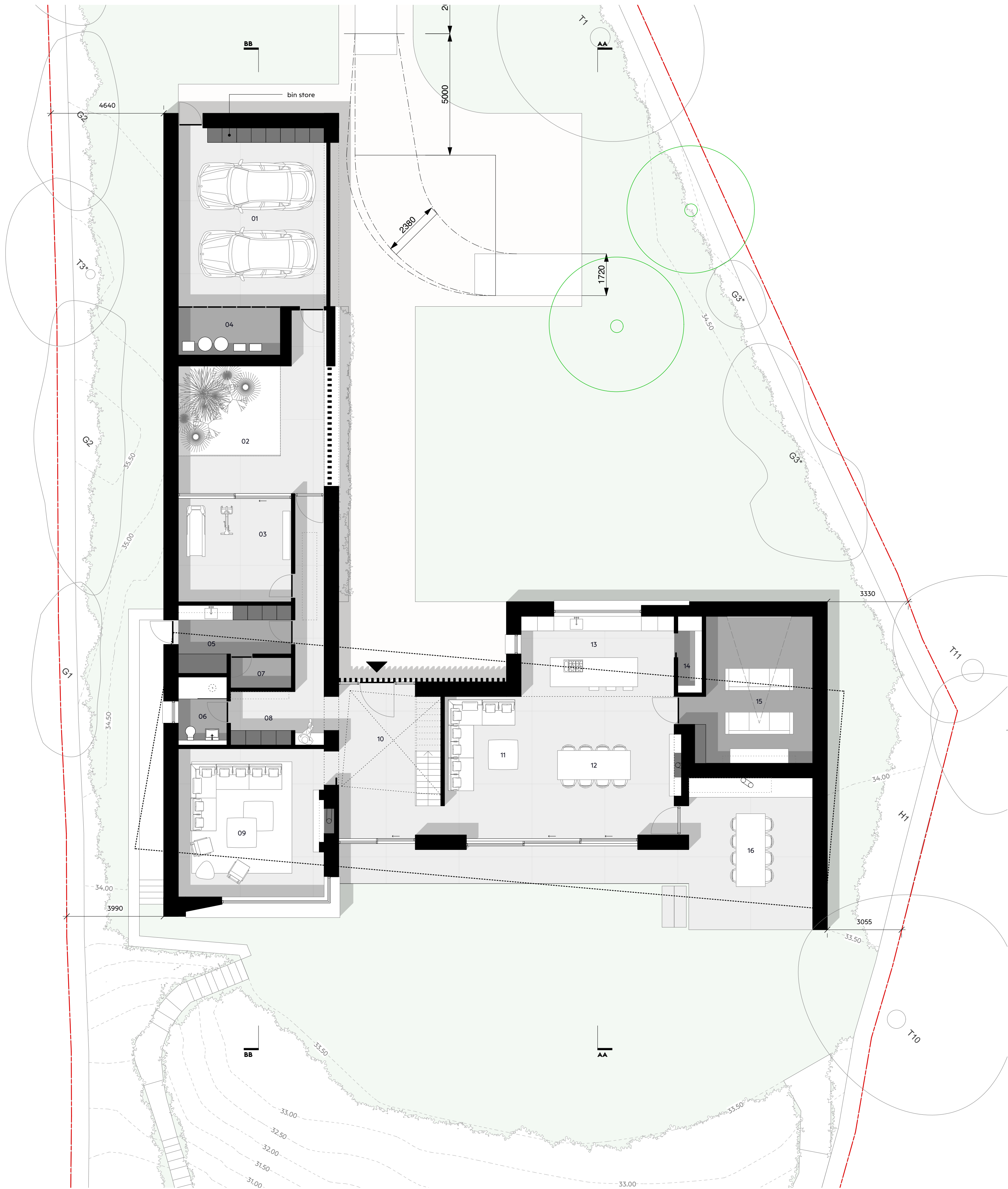
GROUND FLOOR PLAN 1:100 @ A1
