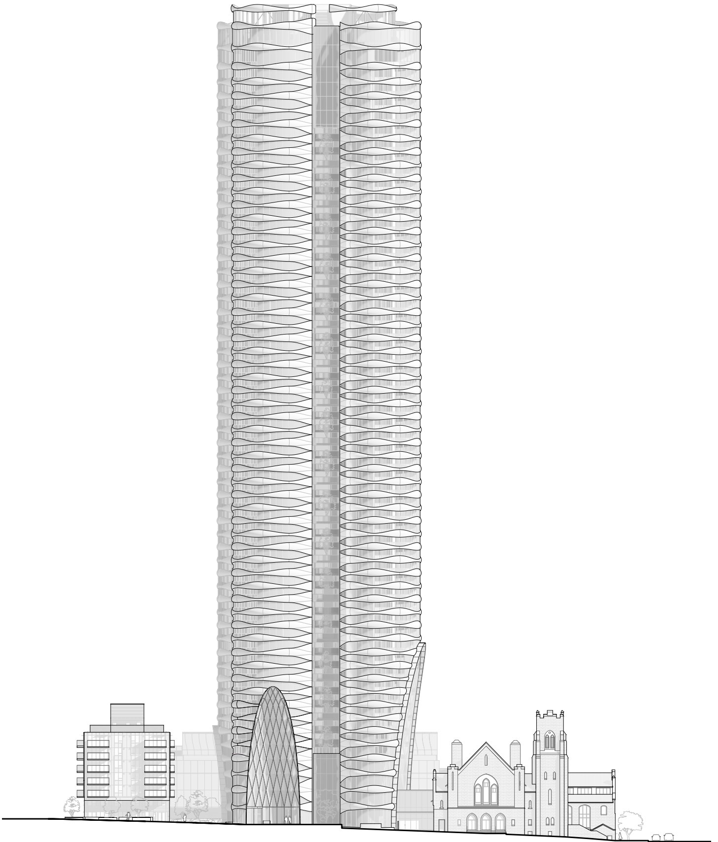
South Elevation
