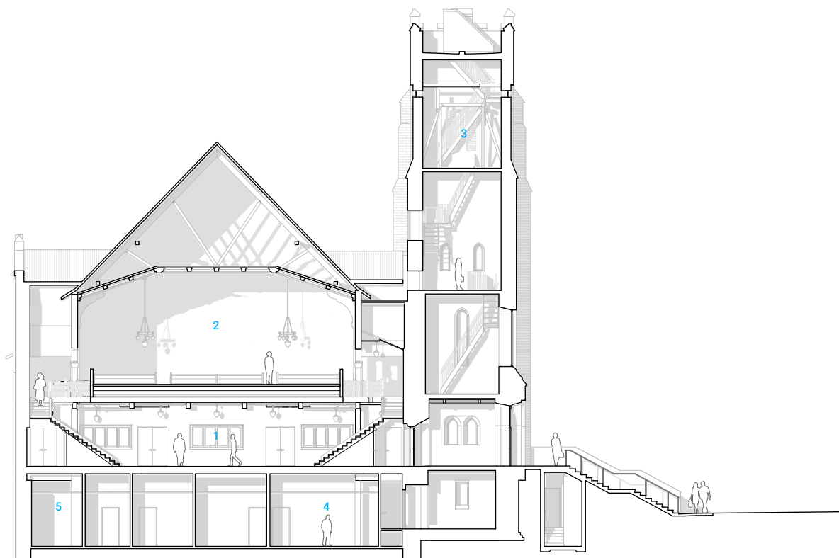
Section F
