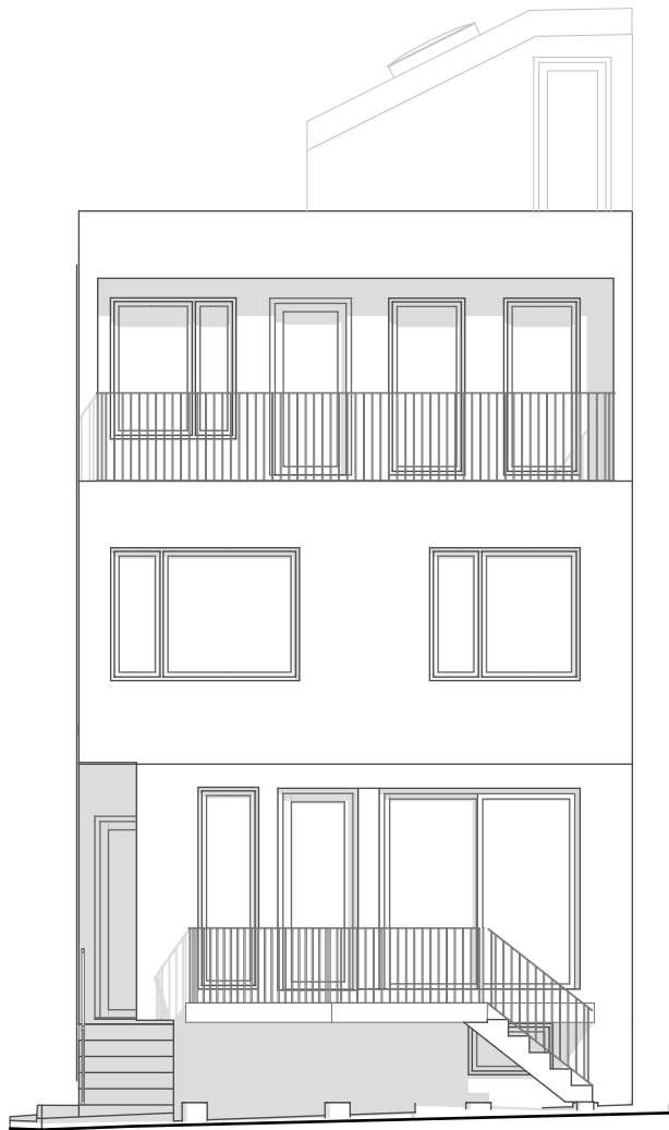
West Elevation
