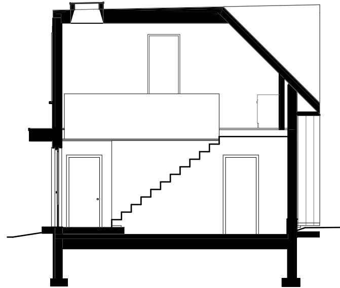
Section
